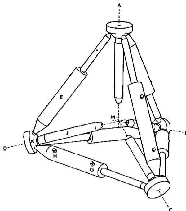
Fig. 3 A hydraulically powered Ram-In-Tie-Bar tetrahedral press
