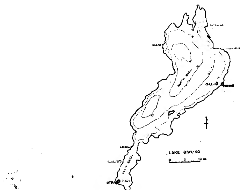
Fig. 1. Map of Lake Biwa-ko. The mark \odot indicates the location of the observation sites, and the mark \otimes the position of the mesh point of the numerical experiments in Table 2.
