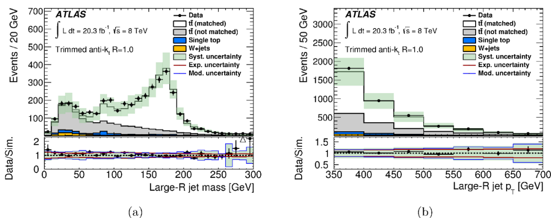
Figure 1. Detector-level distributions of variables reconstructed in events passing the signal-sample selection ( t\bar{t} ) with at least one trimmed anti- k_t R = 1.0 jet with p_T > 350 GeV. Shown in (a) is the mass and in (b) the transverse momentum of the highest- p_T anti- k_t R = 1.0 jet. The vertical error bar indicates the statistical uncertainty of the measurement. Also shown are distributions for simulated SM contributions with systematic uncertainties (described in section 6) indicated as a band. The t\bar{t} prediction is split into a matched part for which the large- R jet axis is within \Delta R = 0.75 of the flight direction of a hadronically decaying top quark and a not matched part for which this criterion does not hold. The ratio of measurement to prediction is shown at the bottom of each subfigure and the error bar and band give the statistical and systematic uncertainties of the ratio, respectively. The impacts of experimental and t\bar{t} modelling uncertainties are shown separately for the ratio.
