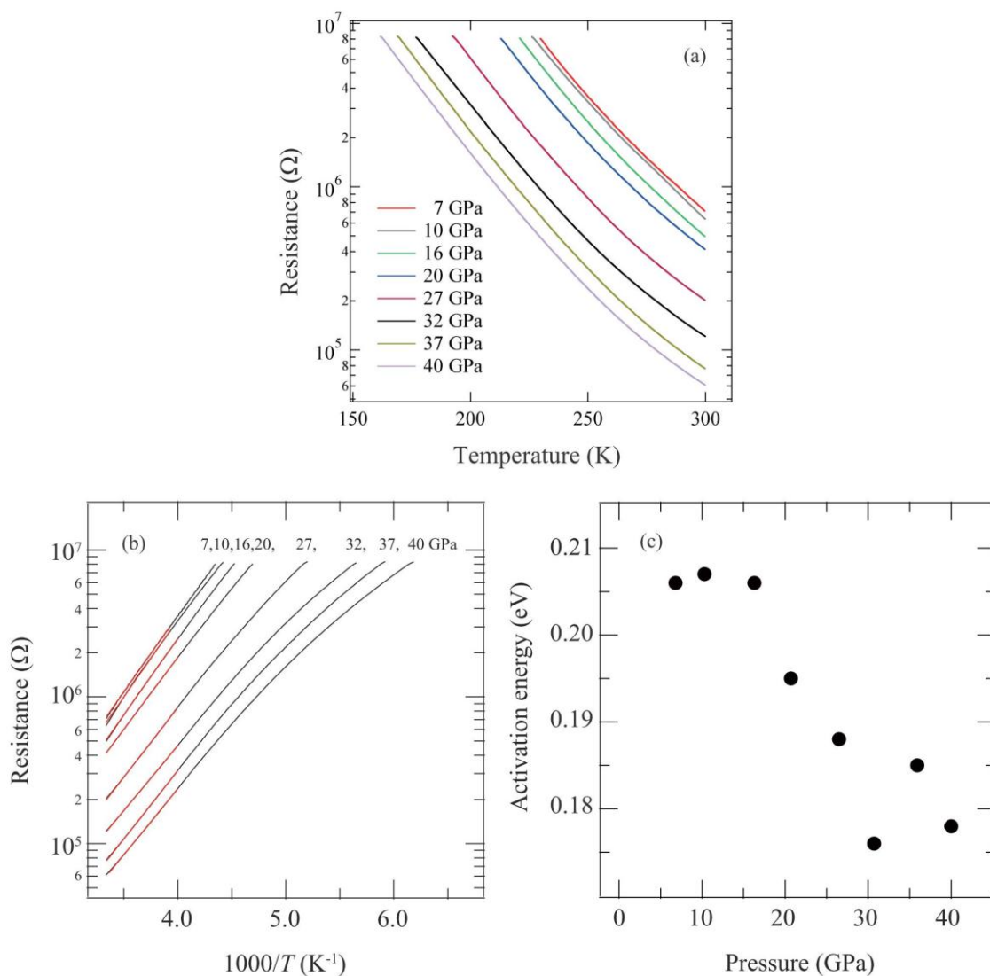
Figure 5.13. (a) Temperature dependence of the electrical resistance under various pressures for Sr_2CuO_3 . (b) Room temperature electrical resistance as a function of 1000/T for Sr_2CuO_3 . Red lines represent Arrhenius plots performed above 250 K. (c) Activation energy as a function of P .
