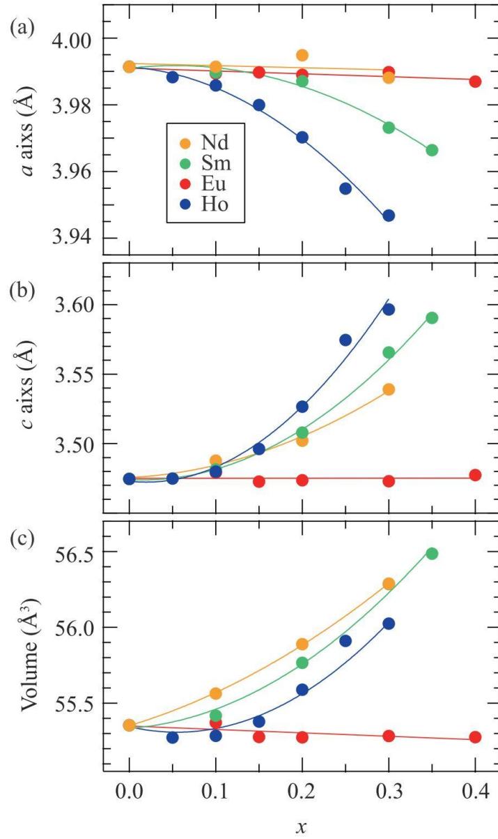
Figure 3.4. The lattice parameters (a, b) and the volume (c) for (\text{Sr}_{1-x}\text{Ln}_x)\text{FeO}_{2+\delta} ( \text{Ln} = \text{Nd} (yellow), \text{Sm} (green), \text{Eu} (red), \text{Ho} (blue)) as a function of lanthanide doping x . The lines are guides to the eye. The data for x = 0.0 are taken from the previous study [3].
