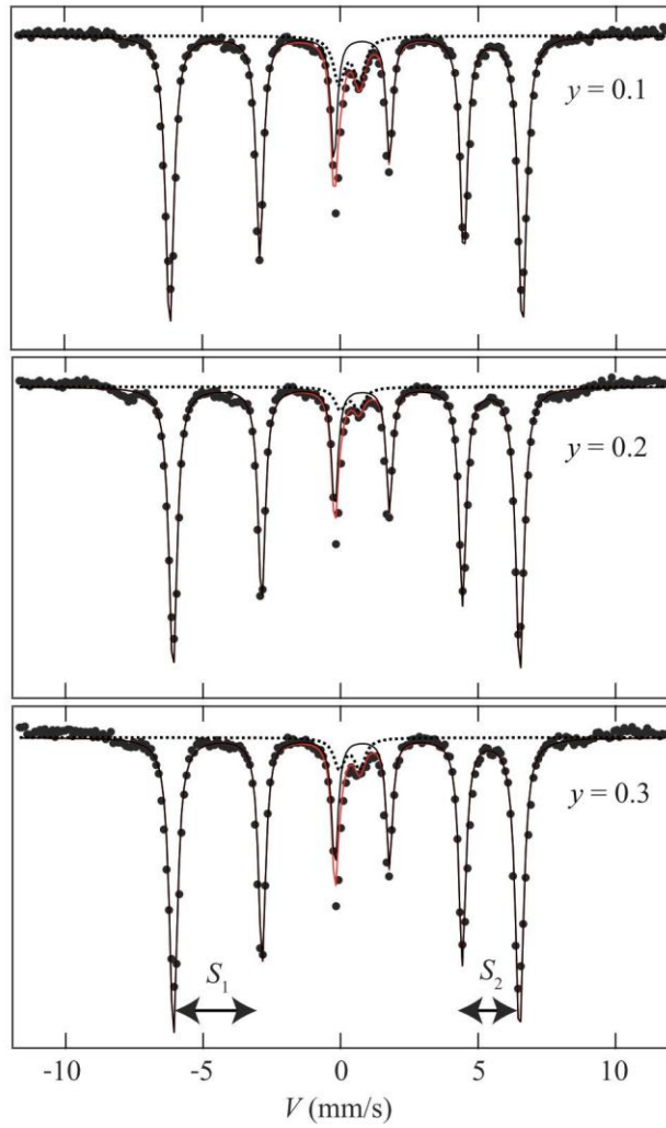
Figure 1.7. Mössbauer spectrum for (\text{Sr}_{1-y}\text{Ba}_y)\text{FeO}_2 ( y = 0.1, 0.2, 0.3 ) at room temperature. Circles denote the experimental data. A black solid line is the spectrum for (\text{Sr}_{1-y}\text{Ba}_y)\text{FeO}_2 and a broken line is that from an overreduced, decomposed impurity formed during the hydride reaction. A red line represents a total fit. S_1 and S_2 are the relative shifts of the peaks.
