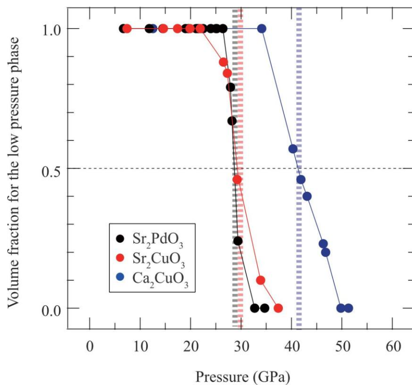
Figure 5.6. Volume fractions of the low and high pressure phases for \text{A}_2\text{MO}_3 . The volume fractions are estimated from the Rietveld refinements. The values of P_s are 29 GPa for \text{Sr}_2\text{PdO}_3 , 30 GPa for \text{Sr}_2\text{CuO}_3 , and 41 GPa for \text{Ca}_2\text{CuO}_3 .
