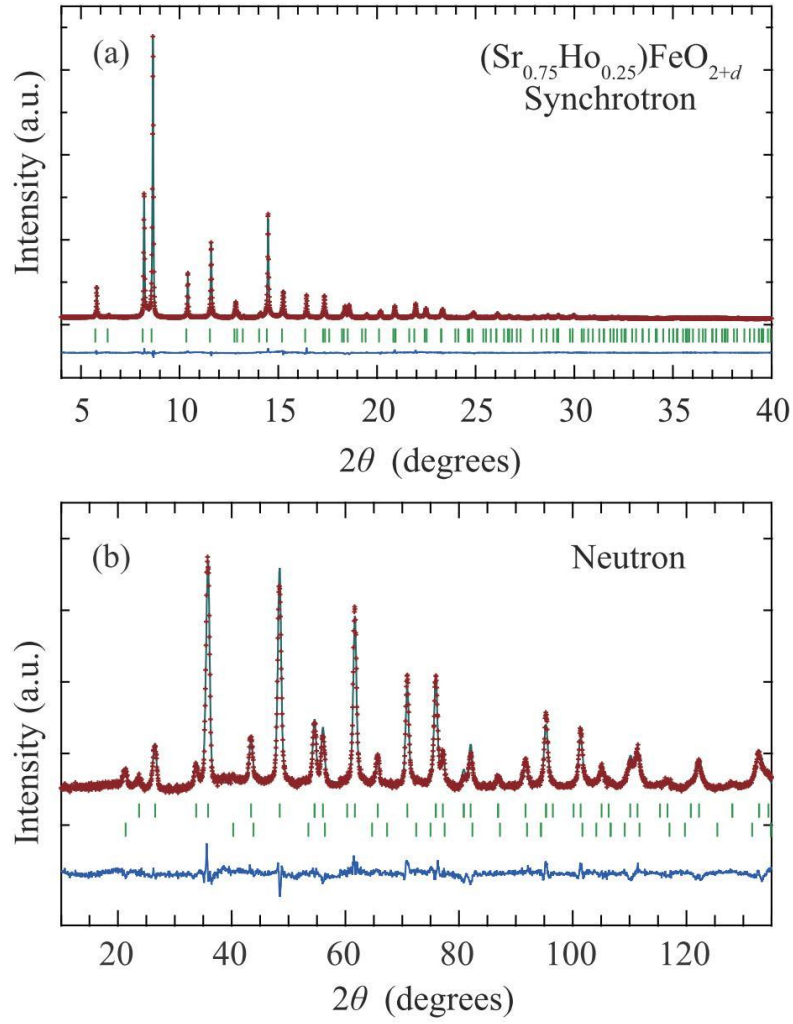
Figure 3.8. (a) Structural characterization of (\text{Sr}_{0.75}\text{Ho}_{0.25})\text{FeO}_{2.125} by Rietveld refinement of synchrotron XRD data at room temperature ( R_p = 3.32\% , R_{wp} = 2.40\% , R_I = 6.16\% , R_F = 6.17\% ), and (b) that of neutron diffraction data at room temperature ( R_p = 5.59\% , R_{wp} = 4.88\% , R_I = 6.61\% , R_F = 3.71\% ). The upper and lower ticks in (b) correspond to the position of the calculated structural and magnetic Bragg peaks.
