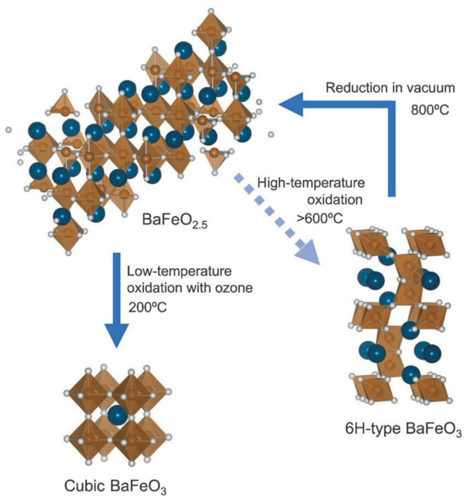
Figure 6.1. Synthetic route for cubic \text{BaFeO}_3 . Ba Blue, Fe brown, O white.
