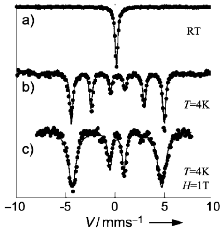
Figure 6.3. Mössbauer spectra of BaFeO 3 taken at room temperature (a) and 4 K (b). The spectrum (c) was obtained from a sample enriched with 57 Fe at 4 K in an external field of 1 T applied parallel to the \gamma -ray beam. The peaks of this spectrum are broadened because of the saturation effect arising from the enrichment. Dotted lines: experimental data points, solid lines: best-fit curves.
