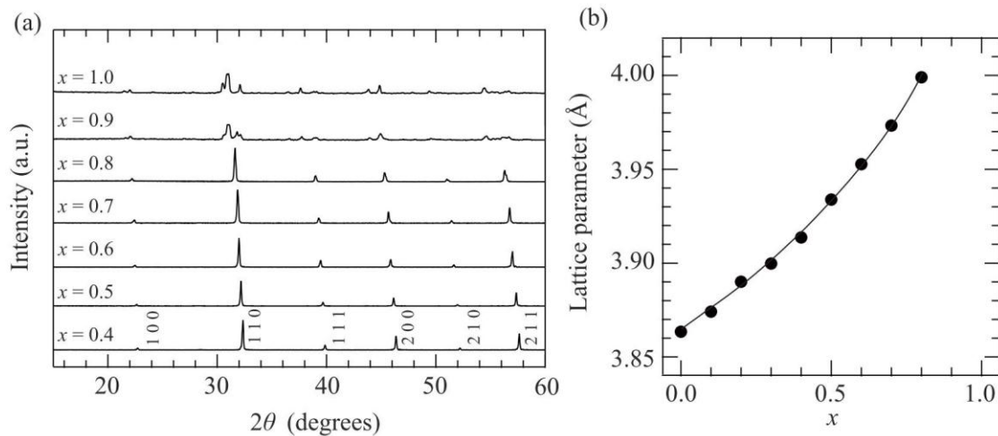
Figure 2.2. (a) XRD patterns of the precursors before reduction. The patterns for x = 0.4, 0.5, 0.6, 0.7 , and 0.8 could be assigned as cubic perovskite (\text{Sr}_{1-x}\text{Ba}_x)\text{FeO}_{3-\delta} ( \delta < 0.5 ), and those for x = 0.9 and 1.0 could be assigned as (\text{Sr}_{1-x}\text{Ba}_x)\text{FeO}_{2.5} with a monoclinic \text{BaFeO}_{2.5} structure [23]. (b) Lattice parameters of (\text{Sr}_{1-x}\text{Ba}_x)\text{FeO}_{3-\delta} ( 0 \leq x \leq 0.8 ). The lattice parameters for x = 0.0 - 0.3 were those obtained from previous studies [26, 29]. The solid line is a guide to the eye. The XRD patterns for x = 0.9 and 1.0 are readily indexed on the basis of a monoclinic unit cell with lattice parameters a = 6.978(4) \text{ \AA} , b = 11.015(7) \text{ \AA} , c = 23.117(16) \text{ \AA} , \beta = 98.22(4)^\circ , V = 1758.6(19) \text{ \AA}^3 for x = 0.9 and a = 6.950(1) \text{ \AA} , b = 11.555(2) \text{ \AA} , c = 23.567(3) \text{ \AA} , \beta = 97.53(1)^\circ , V = 1876.3(5) \text{ \AA}^3 for x = 1.0 .
