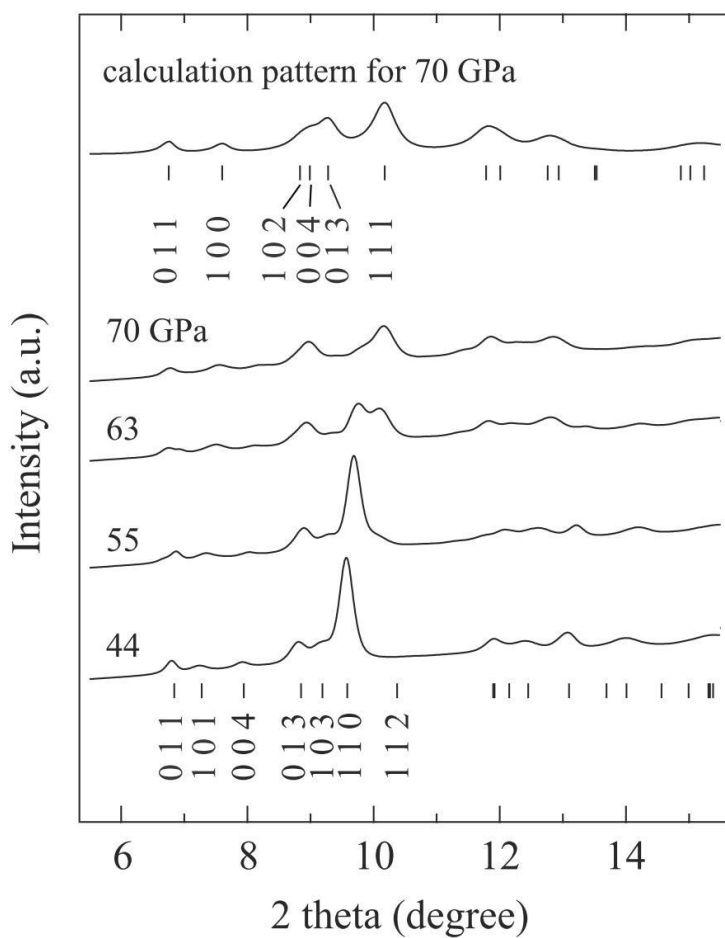
Figure 5.11. Powder synchrotron XRD patterns of \text{LaSrNiO}_{3.4} under high pressures collected at room temperature. The data at 44 GPa were indexed by the I -centered orthorhombic unit cell, while those at 70 GPa by the A -centered orthorhombic unit cell. The ticks represent the positions of the allowed Bragg reflections. The calculation pattern for 70 GPa is obtained by the expected high pressure structure.
