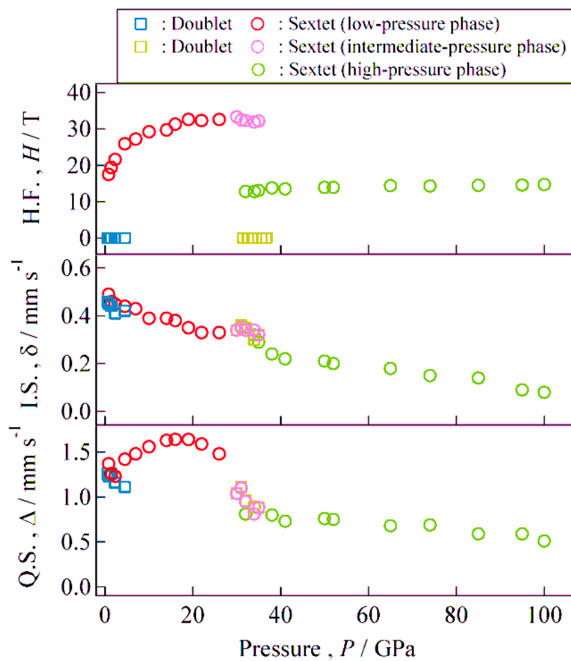
Figure 4.3. Pressure dependence of Mössbauer parameters of \text{Sr}_3\text{Fe}_2\text{O}_5 , H_{\text{hf}} (top), IS (middle), QS (bottom) at RT.
