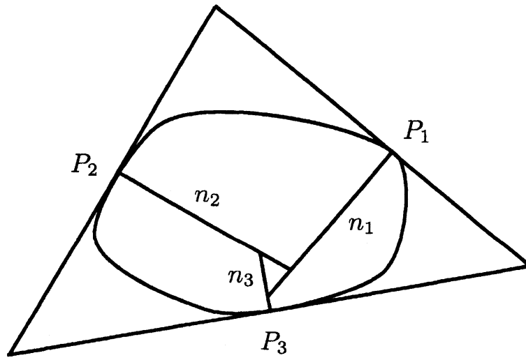
Figure 3: Lines n_1, n_2, n_3 are rotated.
