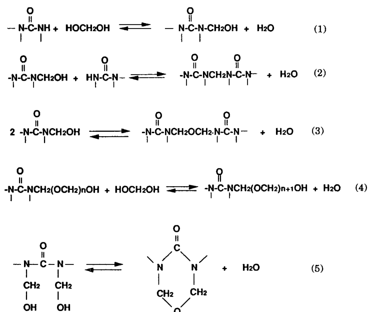
Fig. 2.1. Urea-formaldehyde polymelization and cure reaction.
