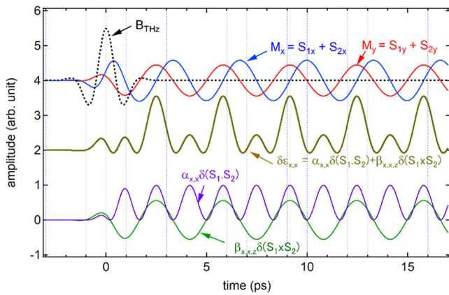
Fig. 3 Numerically calculated waveforms. THz magnetic field: B_{\text{THz}} (black dashed curve), macroscopic magnetization: M_x (blue) and M_y (red), dielectric function \varepsilon_{xx} (dark yellow) and its constituent terms: dot- (violet) and cross product terms (green). Each curve is offset for clarity.
