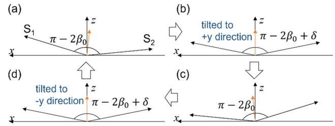
Fig. 4 Schematic representation of the intra-angle modulation of the spin canting angle during the qFM precession. Each panel corresponds to t = 1.6 ps a , t = 2.5 ps b , t = 3.3 ps c , and t = 4.1 ps d in Fig. 3.
