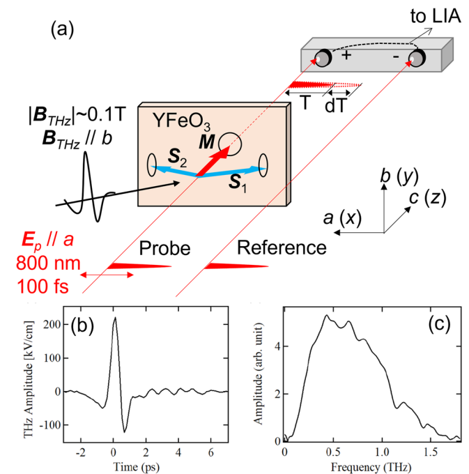
Fig. 1 Schematic of the intense THz pump-induced magnetorefractive measurement. a Experimental setup. The blue and red arrows indicate the sublattice magnetizations \mathbf{S}_{1,2} and net magnetization \mathbf{M} , respectively. RT Room temperature, BPD Balanced photodetector, LIA lock-in amplifier. b Typical waveform of the THz electric field measured with electrooptic sampling in a GaP (110) single crystal with 400 μm thickness. c Fourier spectrum of b .
