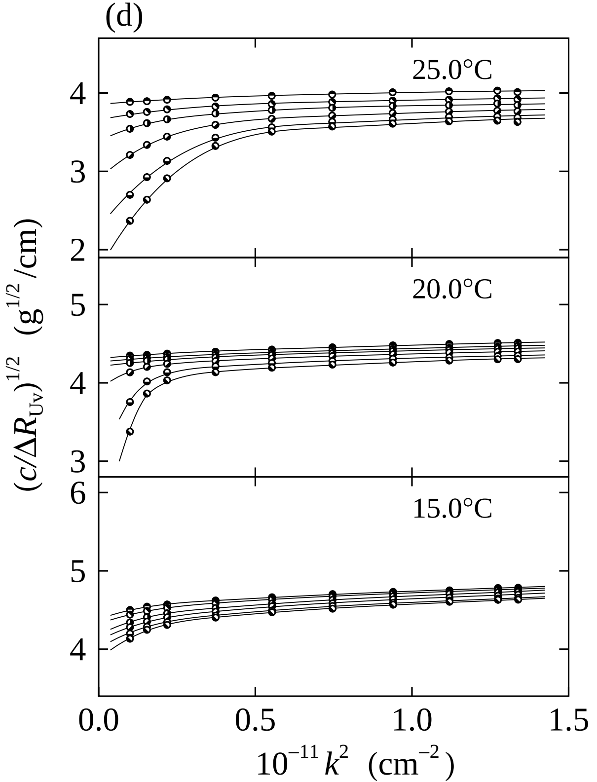
Figure 5.4(d). Plots of (c/\Delta R_{UV})^{1/2} against k^2 for the aqueous PNIPA solution of the sample T7 at w = 1.360\% at 15.0, 20.0, and 25.0 °C. The half-filled circles represent the experimental values with their direction distinguishing the values at t_e \simeq 1 \text{ h} ( \odot ), 3 h ( \bullet ), 6 h ( \ominus ), 12 h ( \odot ), 24 h ( \ominus ), and 36 h ( \bullet ) from top to bottom, and the solid curves connect smoothly the data points.
