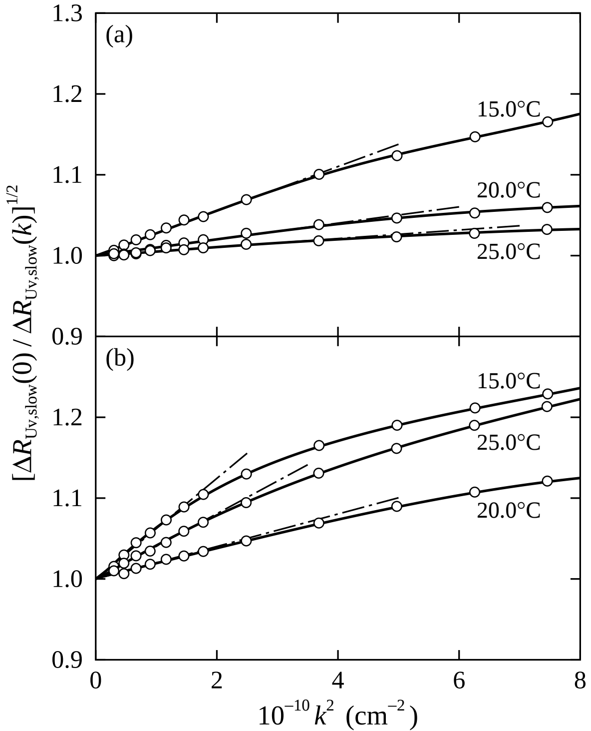
Figure 5.7. Plots of [\Delta R_{\text{UV,slow}}(0)/\Delta R_{\text{UV,slow}}(k)]^{1/2} against k^2 for the aqueous solutions of the sample L7 at w = 1.35\% (a) and of the sample T7 at w = 1.36\% (b), at 15.0, 20.0, and 25.0 °C and at t_e \simeq 36 h. The unfilled circles represent the experimental values and the solid curves connect smoothly the data points. The dot-dashed line segment associated with each curve indicates its initial tangent.
