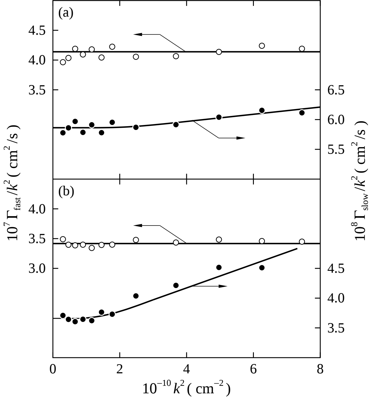
Figure 5.6. Plots of \Gamma_{\text{fast}}/k^2 ( \circ ) and \Gamma_{\text{slow}}/k^2 ( \bullet ) against k^2 for the aqueous solutions of the sample L7 at w = 1.35\% (a) and of the sample T7 at w = 1.36\% (b), at 25.0^\circ\text{C} and at t_e \simeq 36 h. The horizontal line associated with each plot of \Gamma_{\text{fast}}/k^2 indicates the mean of the experimental values and the curve associated with each plot of \Gamma_{\text{slow}}/k^2 connects smoothly the data points.
