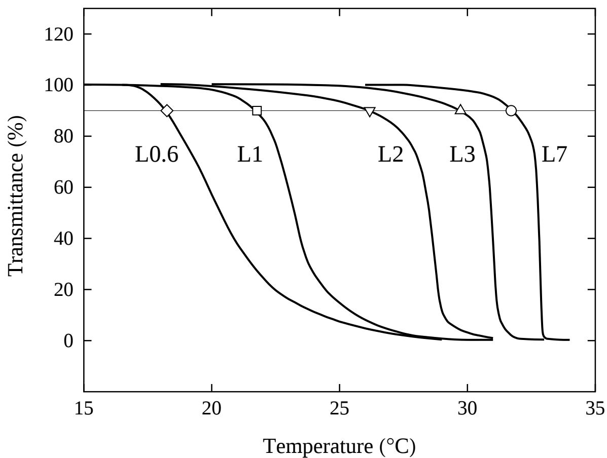
Figure 4.4. Temperature dependence of the transmittance of light passing through aqueous solutions of the PNIPA samples L0.6, L1, L2, L3, and L7 at w = 5.03, 4.97, 4.94, 4.93 , and 4.94 %, respectively, the symbols \diamond , \square , \nabla , \triangle , and \circ representing the respective cloud points (see the text).
