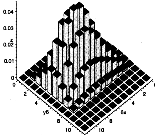
Fig.1. The exact joint probability function of (X_{10}^{(1)}, X_{10}^{(2)}) in the Example 4.1, given \mathbf{b}_0 = (1, 2, 1, 2) and the addition matrix A .
