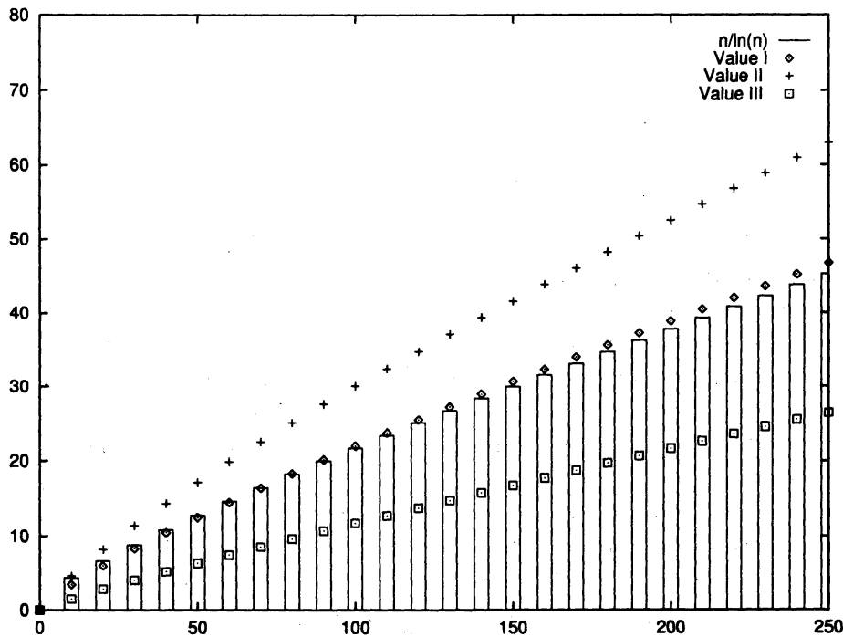
Fig.2. The exact expected values of Y_n , given three initial urn compositions b_0 = (1, 1), (2, 3), (5, 1) and the addition matrix A in Example 4.2. Value I, II, III are, respectively, the values given initial urn compositions b_0 = (1, 1), (2, 3), (5, 1) .
