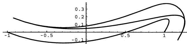
Fig. 6-1. Cubic spline and its spline offset curve composed of three parts with d = 0.2 (Ex.4).
