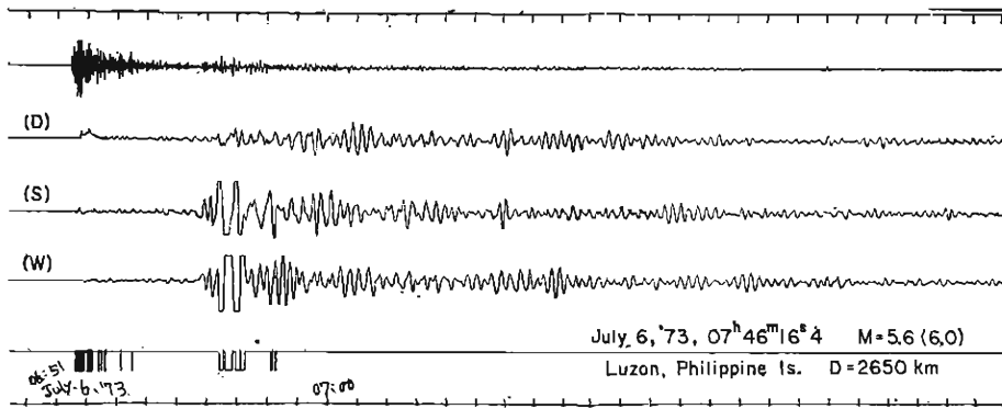
Fig. 10. Analog record of the earthquake of Philippine, July 6, 1973, 07^h 46^m 16^s , \Delta = 2650 km, M = 5.6 .
