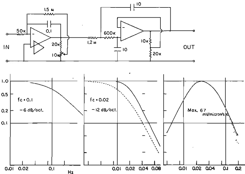
Fig. 7. Upper part; amplifier and filter circuit.
