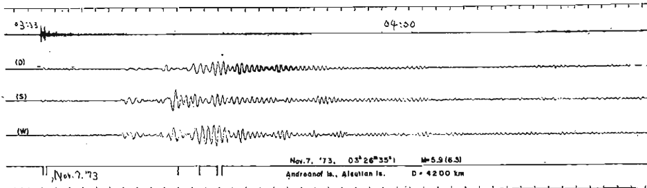
Fig. 11. Analog record of the earthquake of Aleutian Is., Nov. 7, 1973, 03^h 26^m 35^s , \Delta \approx 4200 km, M = 5.9 .
