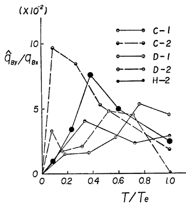
Fig. 4 Comparison of present data with previous ones of an intensity index of lateral sediment transport ( \hat{q}_{By}/q_B )
