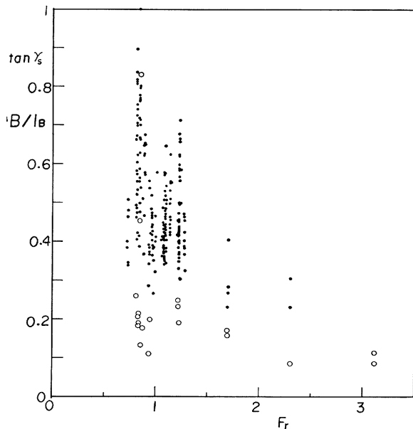
Fig. 6 Directions of oblique edges on a sand bed as a function of F_r .
