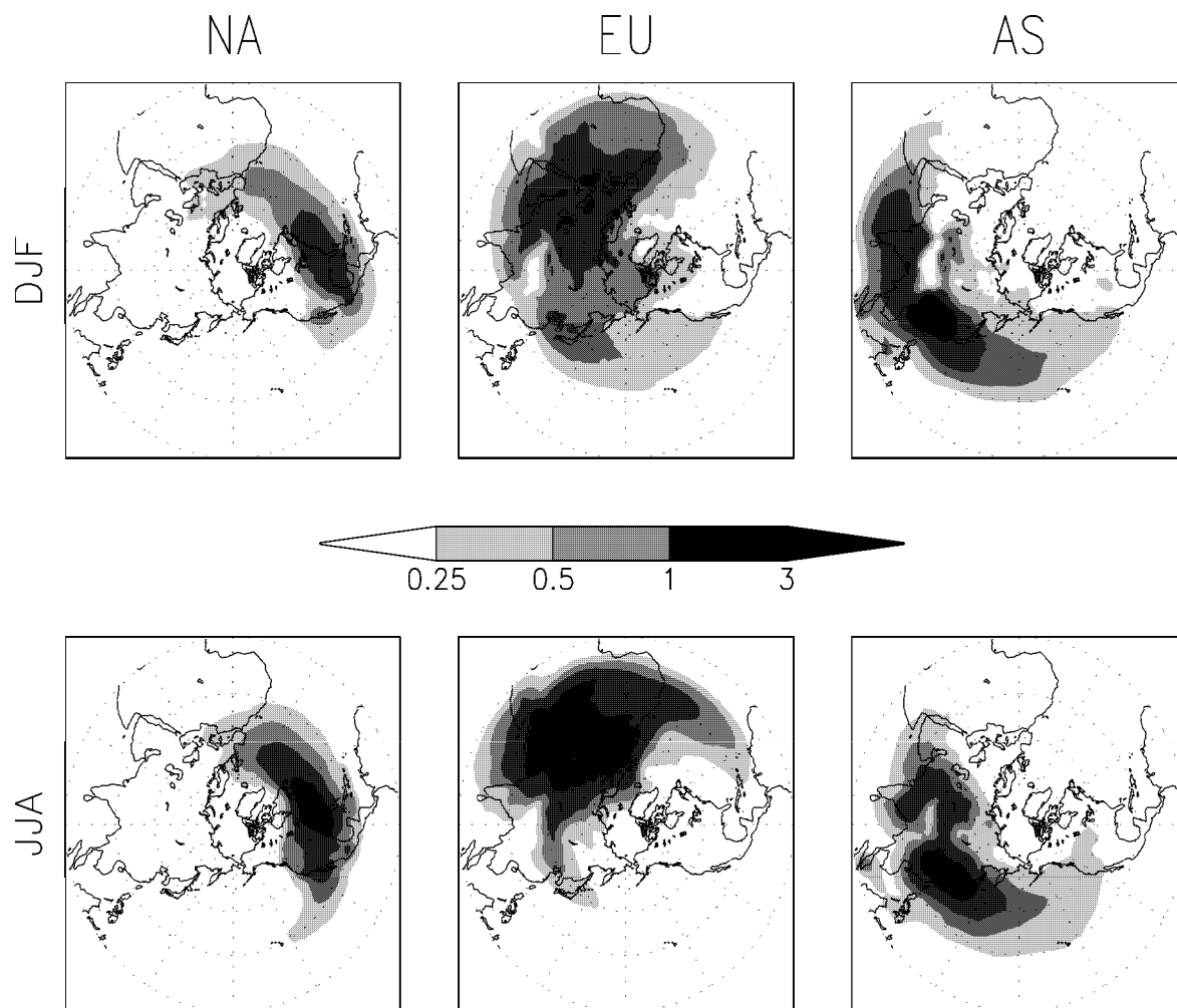
Fig. 2 Seasonally averaged column burdens of the three emission components of sulfate in the Northern Hemisphere. Unit is \text{mgS}/\text{m}^2 .
