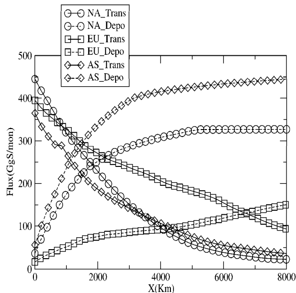
Fig. 9 Seasonally averaged SO_x fluxes of transport through each meridional planes (solid) and deposition in the west side (dashed) in winter. Circles, squares, and daiamonds represent North America (NA), Europe (EU), Asia (AS), respectively. The fluxes are function of the distant from the start point in Fig. 8.
