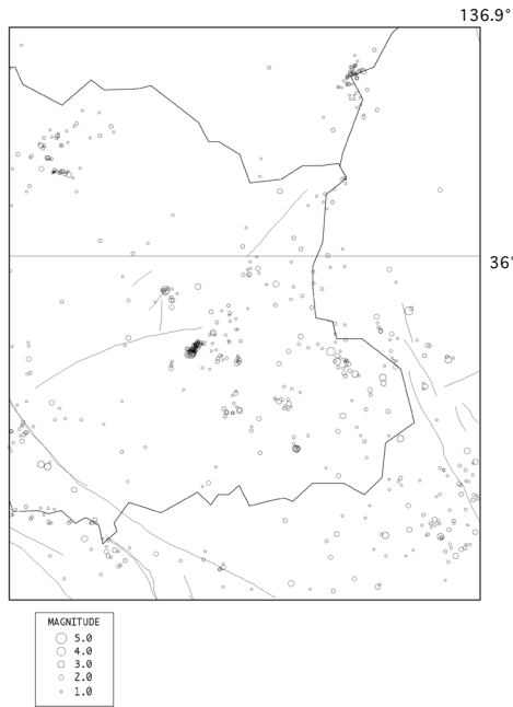
Fig.4.a Epicenter of Earthquakes (M ≥ 1.0, Z ≤ 30km, 2000.1 - 2005.2)
