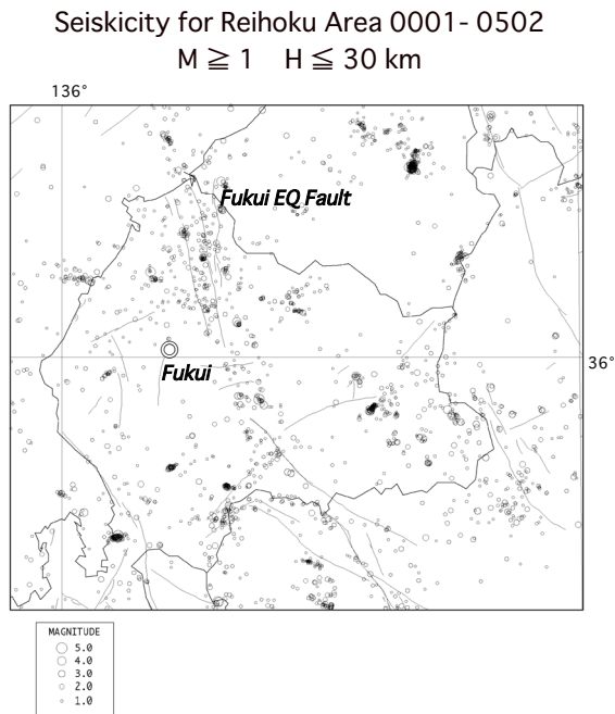
Fig.1 Epicenter of earthquakes (2000.01-2005.02)
