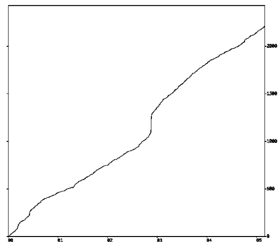
Fig.3 Cumulative number of Fig.1
