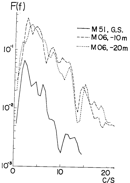
Fig. 12 Velocity Spectra (Matsushiro-so).
