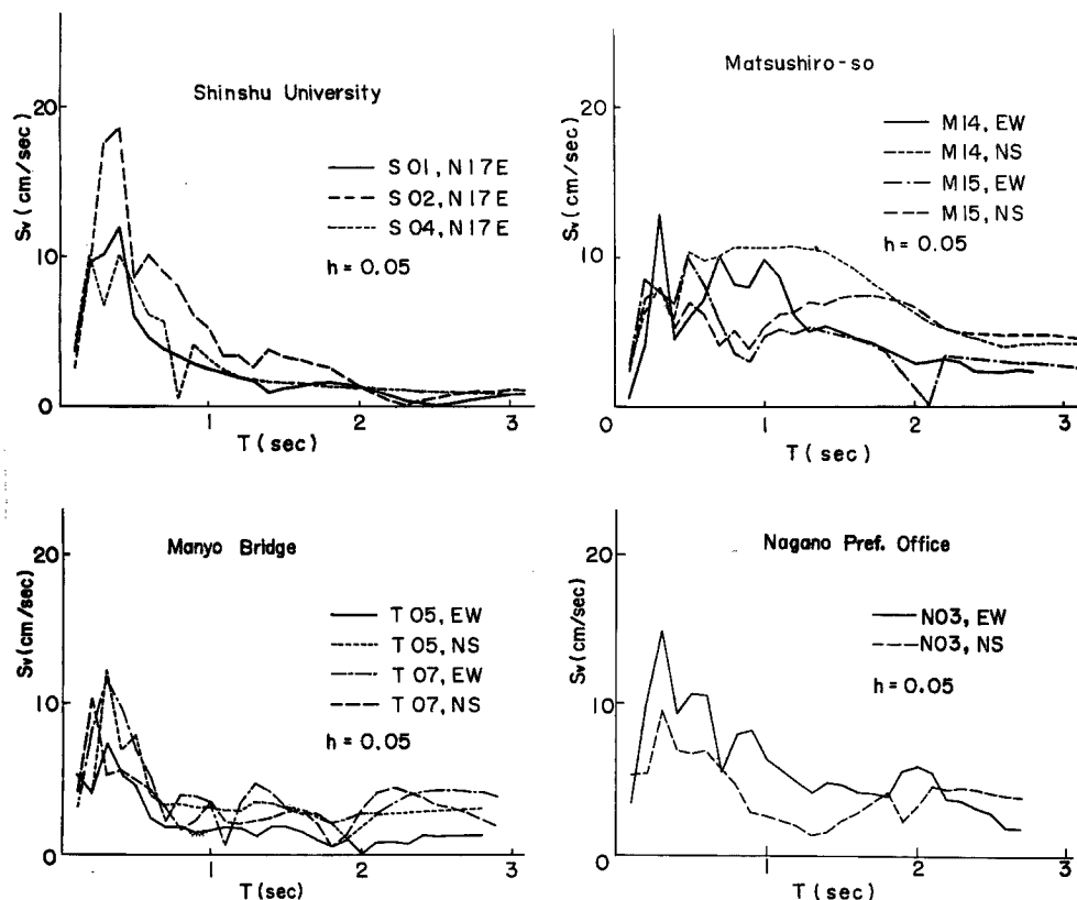
Fig. 13 Velocity Response Spectra of Matsushiro Earthquakes.
