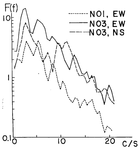
Fig. 9 Acceleration Spectra (Nagano Pref. Office).
