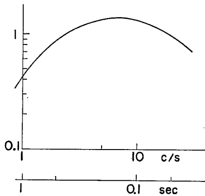
Fig. 15 Frequency Characteristics of Microtremometer.
