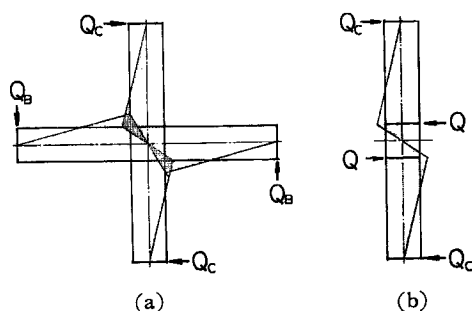
Fig. 1 State of stress in the Connection Panel
