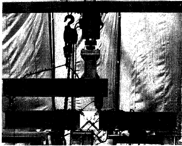
Photo. 1 Experimental Set-up
