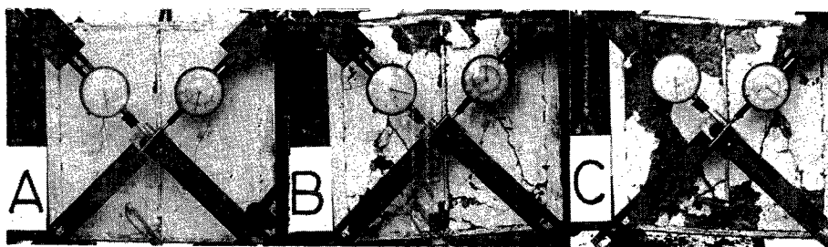
Photo. 4 Deformation Process of SBC 1 -R
