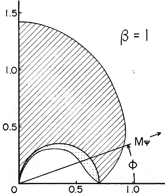
Fig. 2. The curves for the polar plots of M_T as functions of \phi in the case of \beta=1 , where M_T = M \cos \Psi . The shaded region is the instability domain and the dotted region is the overstability domain.
