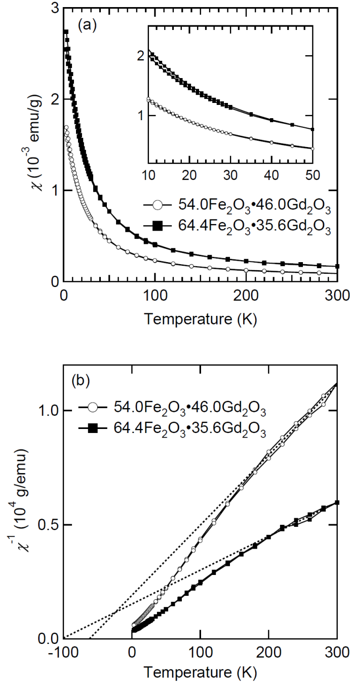
Figure 2.4: Temperature dependence of (a) magnetic susceptibility and (b) inverse magnetic susceptibility for the thin films of the \text{Fe}_2\text{O}_3 - \text{Gd}_2\text{O}_3 system. The inset of Fig. 2.4(a) shows an enlarged view of low temperature regime. The dashed lines in Fig 2.4(b) correspond to the Curie-Weiss law described by Eq. (2.1).
