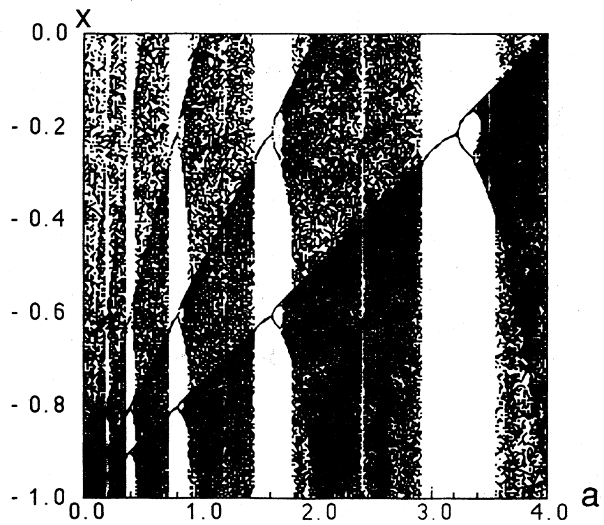
Fig. 11. Bifurcation diagram for Eq. (12), where \alpha = 0 .
