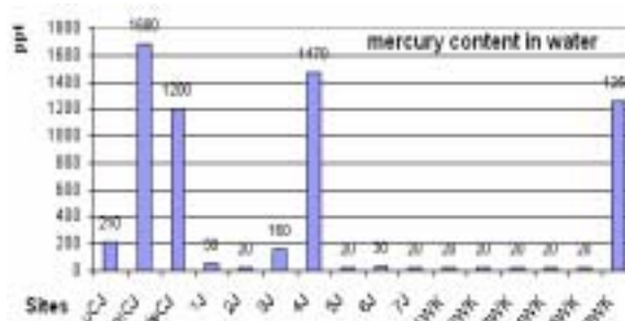
Fig. 6 The comparison of total mercury content in water taken from three different rivers. CJ = central java, J = Jambi, WK = West Kalimantan
