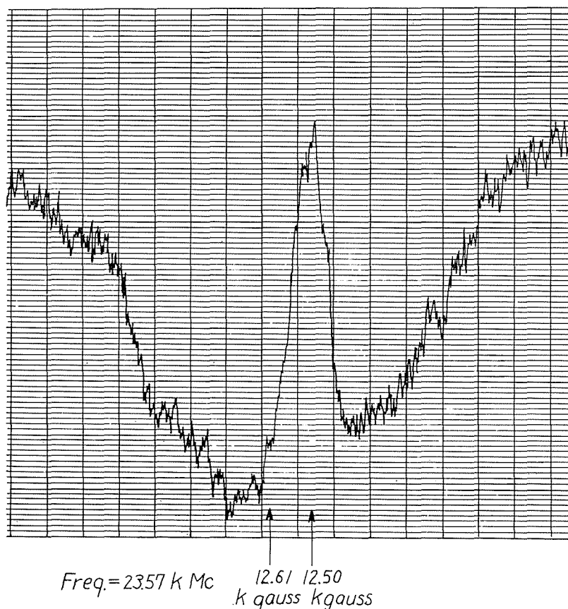
Fig. 10. Recorder trace of an extraordinary signal like 'hole burning' corresponding to w_3 at 1.8°K in 0.3 percent ruby.
