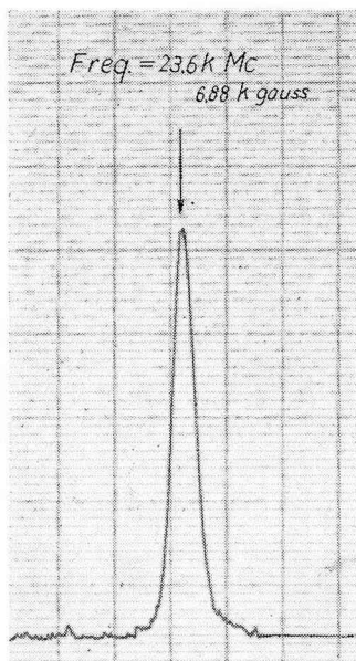
Fig. 8. Typical recorder trace of the signal corresponding to w_e at 1.8^\circ\text{K} in 0.1 percent ruby.
