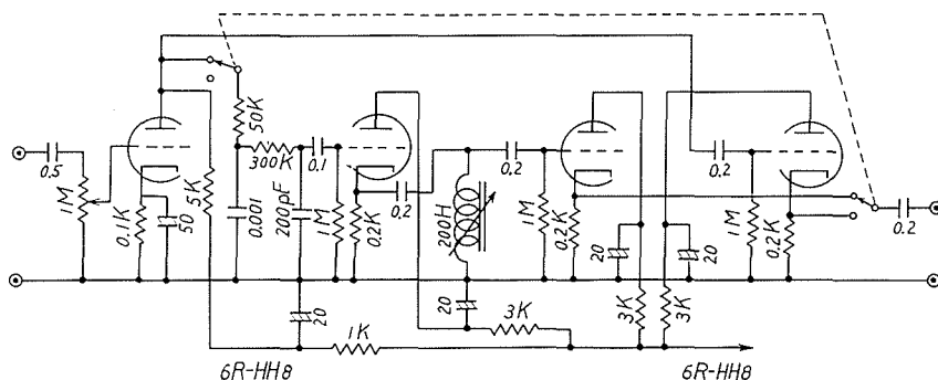
Fig. 6. Circuit diagrams of the preamplifier and filters.
