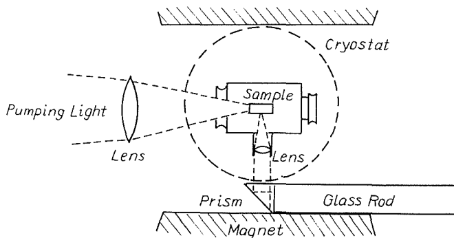
Fig. 7. Location of the helium cryostat and the glass rod in the magnet.
