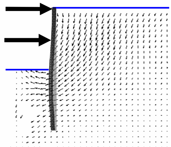
(c) Excavation against a multi-propped wall
