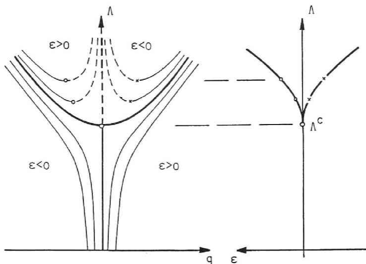
Fig. 1.4.3 Stable Symmetric Point of Bifurcation with Cusp Catastrophe. [25,64] (a) Equilibrium Paths (b) Imperfection Sensitivity Curve
