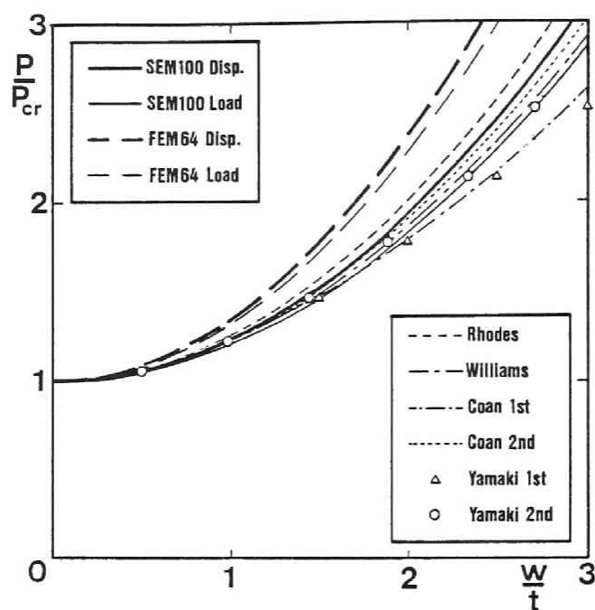
Fig. 4.3.6(a) Postbuckling Equilibrium Paths of Compressed Plate. (i) All Edges Simply Supported.
