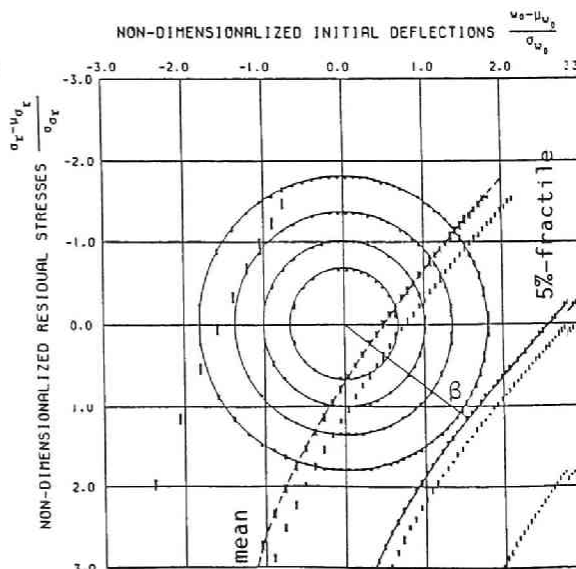
Fig. 2.5.5 Contour Lines of Strength for Compressed Stiffened Plates: R=1.4 , \gamma/\gamma^*=0.5
