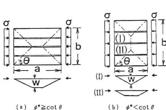
Fig. 2.2.4 Plastic Fold Lines of Failure Mechanisms for Global Buckling Mode.
