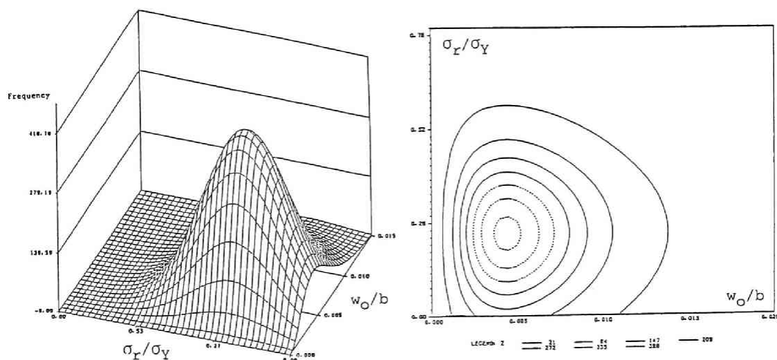
Fig. 2.5.1 Joint Probability Density Function of Residual Stresses and Initial Deflections.
