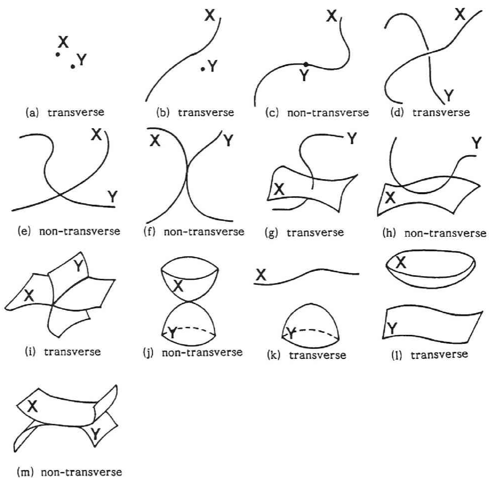
Fig. A.4.3 Some Examples for Transversality. [7]
