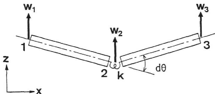
Fig. A.1.2 Flexural Spring between Two Adjacent Elements for Column Model.
