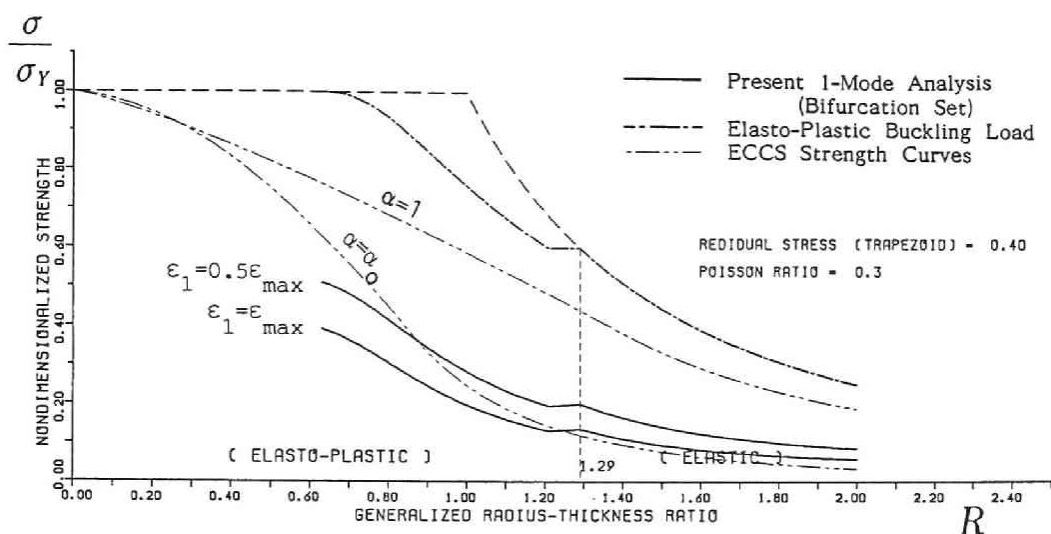
Fig. 3.3.1(c) Ultimate Strength Curves of Compressed Cylindrical Shells with Trapezoidal Residual Stress. 1-Mode Analysis. \sigma_r = 0.4 \sigma_Y
