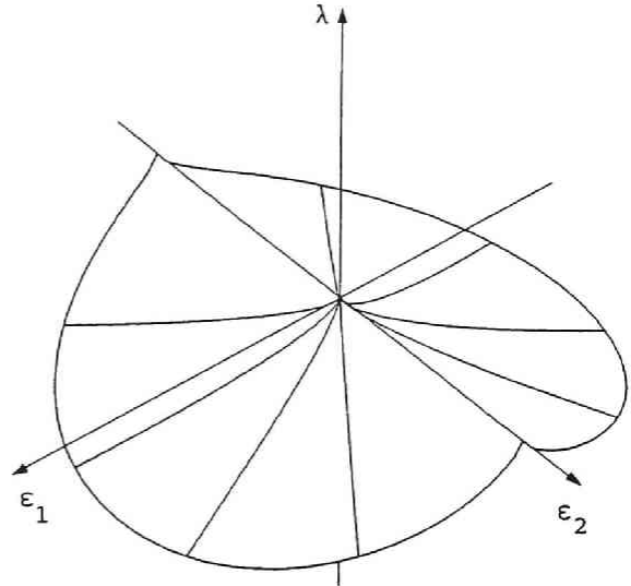
Fig. 2.3.2 Bifurcation Set for Dual Cusp Catastrophe.
