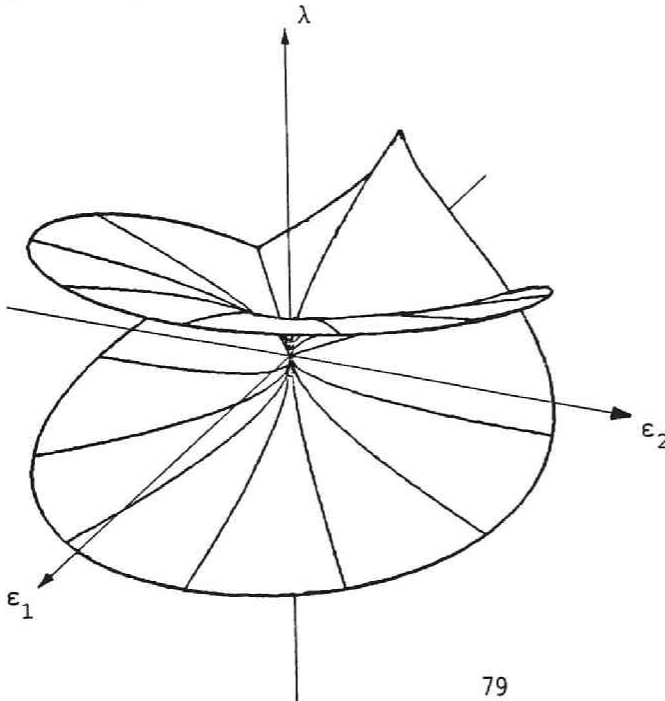
Fig. 2.4.1 Bifurcation Set for Hyperbolic Umbilic Catastrophe with Monoclinal Bifurcation.
