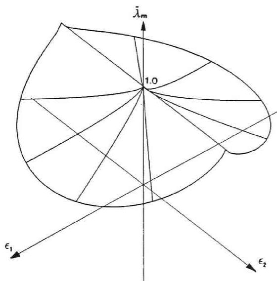
Fig. 3.3.2 Imperfection Sensitivity for Dual Cusp Catastrophe of Unstable Symmetric Model. \kappa = 1.5
