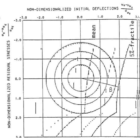
Fig. 2.5.3 Contour Lines of Strength for Compressed Plates: R=1.4
