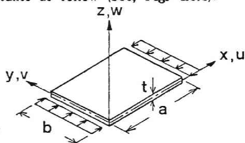
Fig. 4.3.1 Plate Model in Compression.
