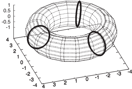
(a) K=400 , M=3 , aligned
