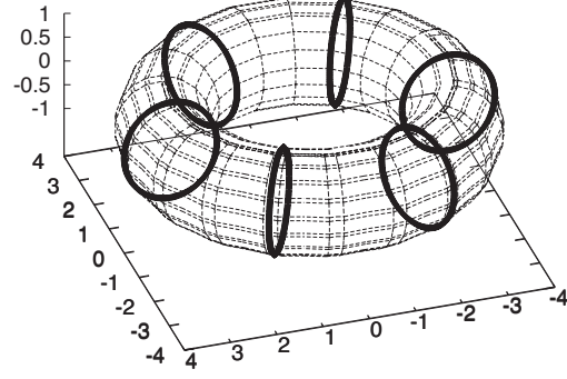
(b) K=800 , M=3 , staggered
