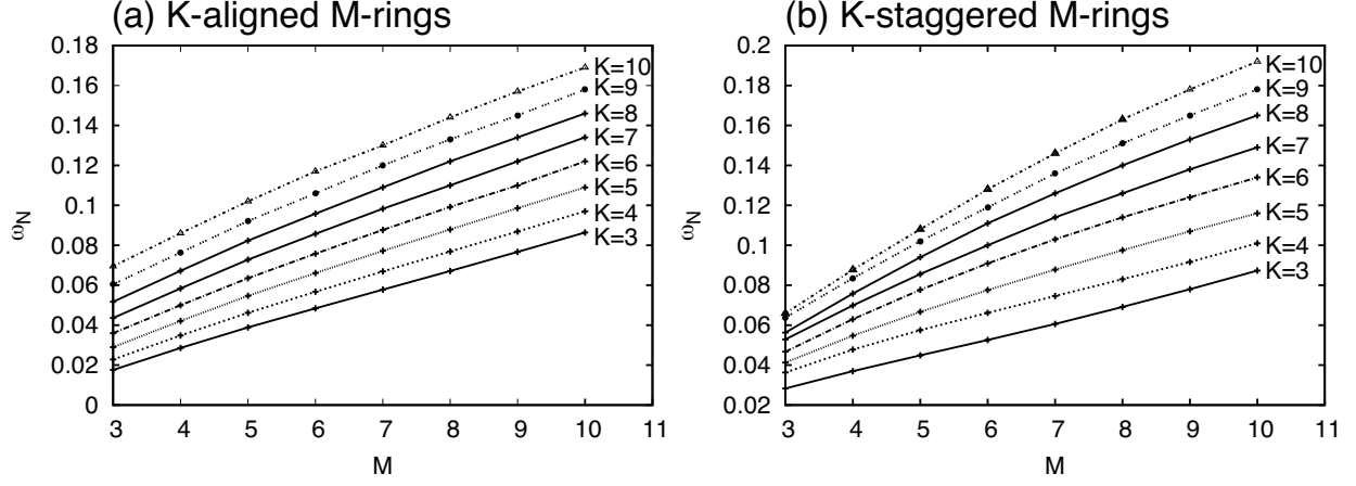
Figure 8: Entropy ratio \omega_N for (a) K -aligned M -rings and (b) K -staggered M -rings. The aspect ratio of the torus is \alpha = 3.0 .
