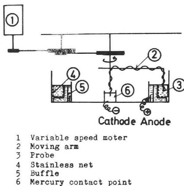
Fig. 5-12 Experimental apparatus.
