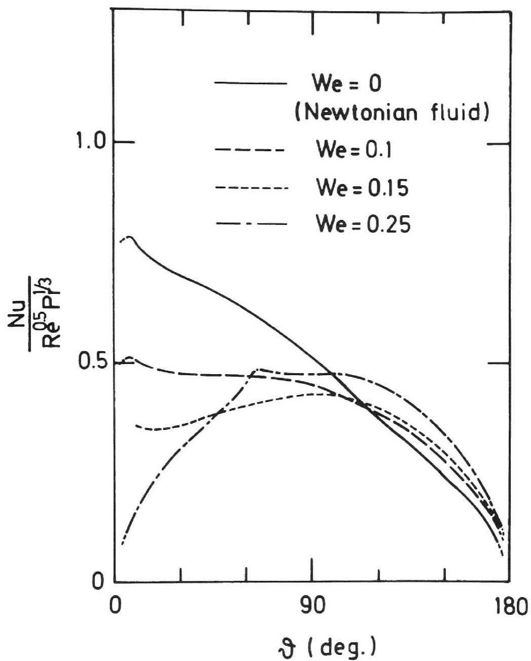
Fig. 5-11-a Distribution of local Nusselt number at Re = 1.0 .
