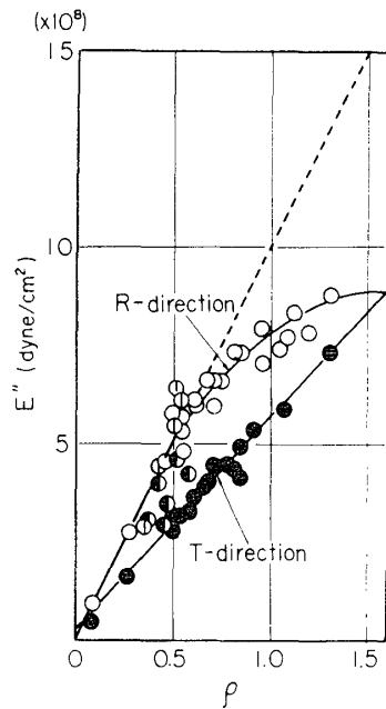
Fig. 6. The relation between E'' and \rho in the transverse direction at 60 kHz. ○ hardwood in R-direction, ⊙ softwood in R-direction, ● hardwood in T-direction, ⊖ softwood in T-direction.
