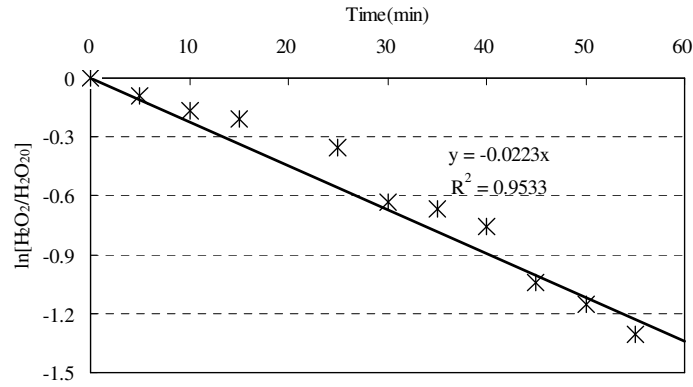
Fig. 3-4 Degradation of H_2O_2 at UV 254 nm
