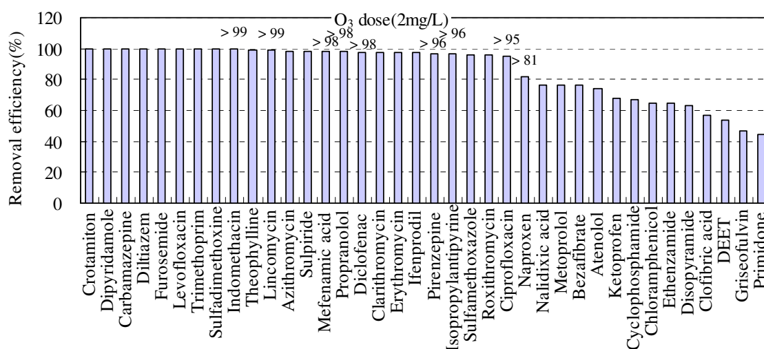
Fig. 6-7 Removal efficiency of the 38 PPCPs during O 3 process (Run 8, contact time: 10 min)
