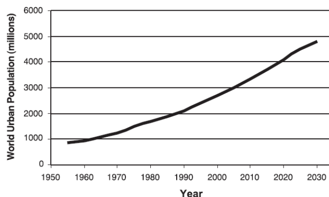
Fig. 2-1 Estimated and Projected Urban Population in the World (U.S. EPA, 2004)
