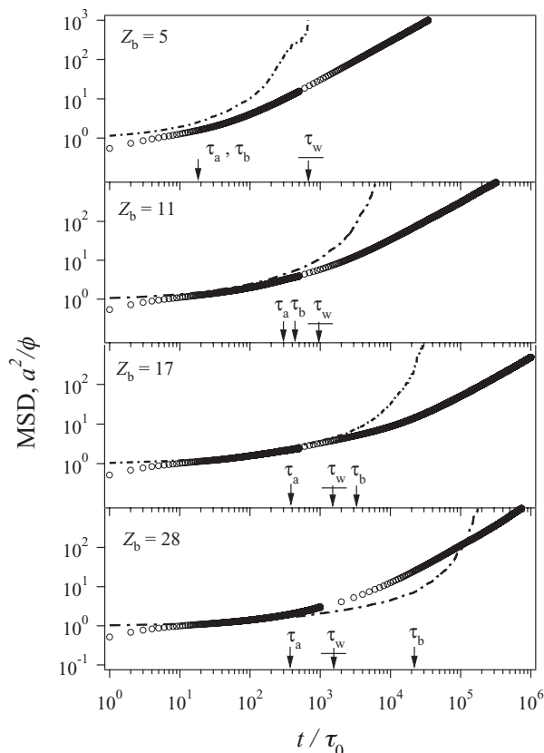
FIG. 8. Mean square displacement MSD of the branch point (circle) and squared mesh size of fully dilated network a'(t)^2 = a^2/\phi(t) (dash-dot curves) for the asymmetric star polymers examined in Fig. 7.
