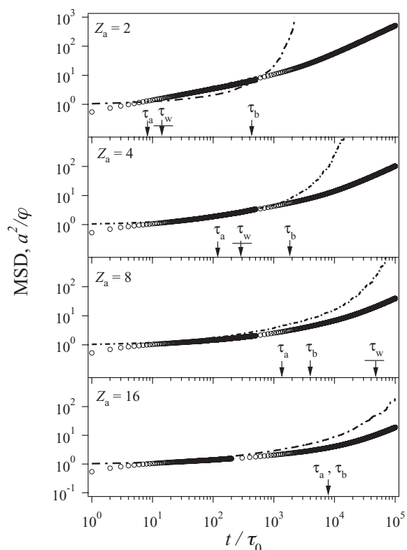
FIG. 6. Mean square displacement MSD of the branch point (circle) and squared mesh size of fully dilated network a'(t)^2 = a^2/\phi(t) (dash-dot curves) for the asymmetric star polymers examined in Fig. 5.
