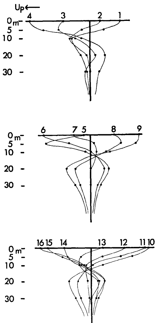
Fig. 10 Amplitude distributions of the wave group II with depth.
