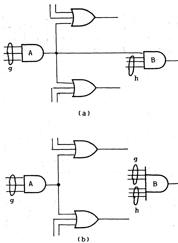
Fig.3.1 Transformation to Normal AND-OR circuit
