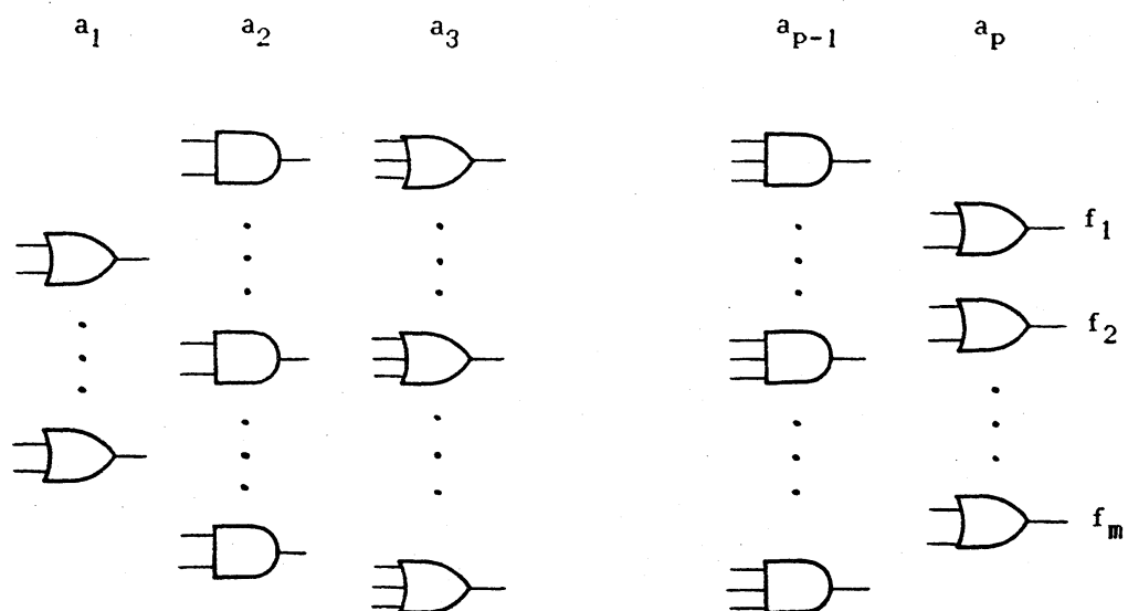
Fig.3.2 Normal AND-OR multi-level Circuit
