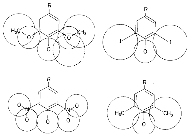
Fig. 3. Diagrams of steric hindrance of dual o -substituted phenoxyl radicals. Fields of van der Waals of iodine, methyl and nitro groups are fixed because of only one single bond (the formers) and the resonanced \pi -electrons (the latter). However, methoxyl group has two single bonds which can rotate around the aromatic C-O bond. Dashed circle shows the nearest position of methoxyl group to the phenoxyl radical but that position is less possible.
