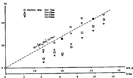
Fig. 18. Unsteady airforce coefficient for B/D=1.0 rectangular cylinder in smooth flow.
