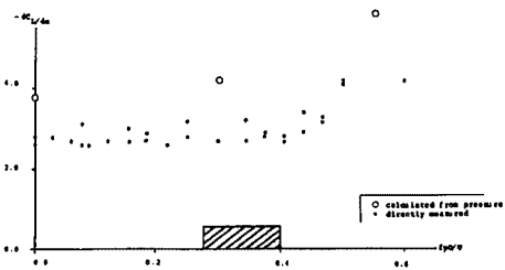
Fig. 9. Gradient of lift coefficient v. s. pulsating frequency for B/D=2.0 rectangular cylinder.
