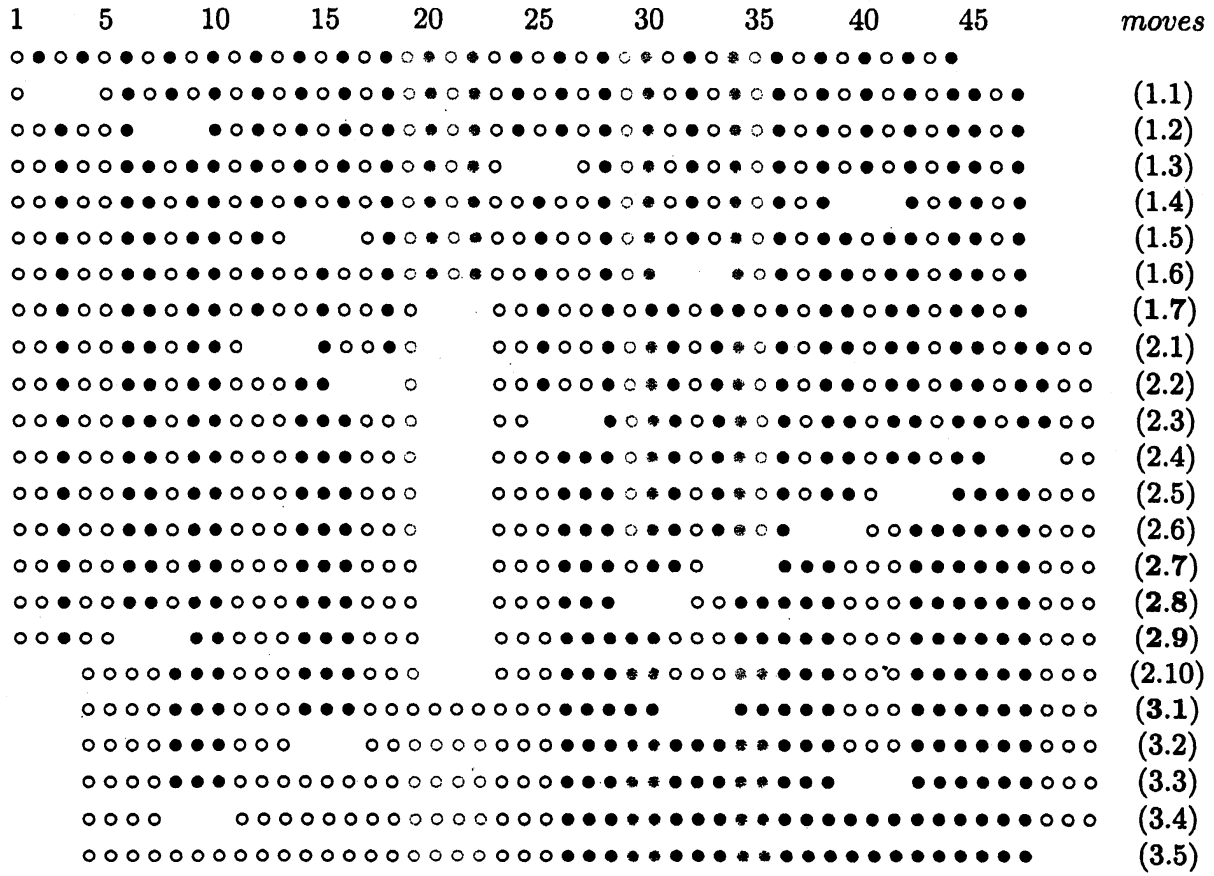
Figure 5: Sorting the alternating 44-string by 22 Berge 3-moves
