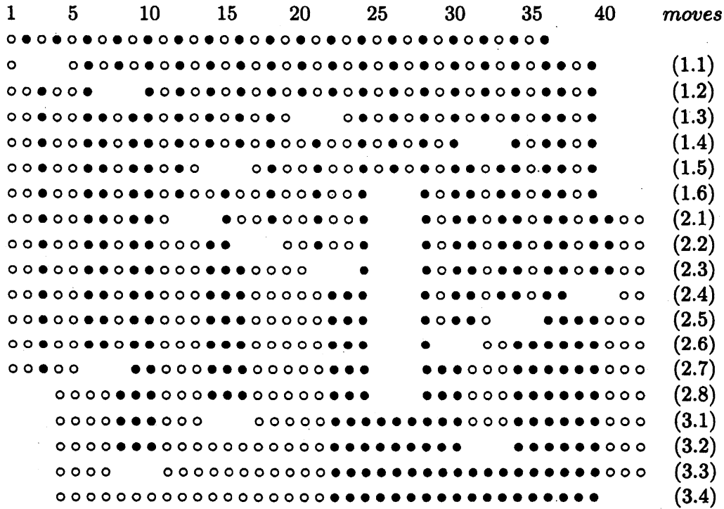
Figure 4: Sorting the alternating 36-string by 18 Berge 3-moves
