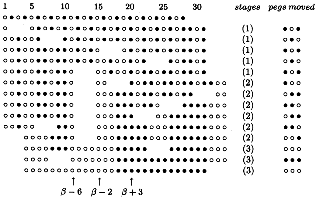
Figure 3: Sorting the alternating 28-string by 14 Berge 3-moves
