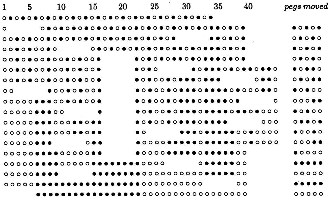
Figure 6: Sorting the alternating 34-string by 17 Berge 5-moves
