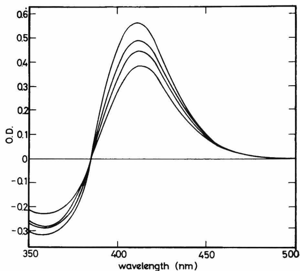
Figure 5 Difference spectra of IAI-C3PVP complex at 25°C. [IAI] = 3.96 \times 10^{-5} M , [C3PVP] = 0.005 - 0.04 \text{ equiv. l}^{-1}
