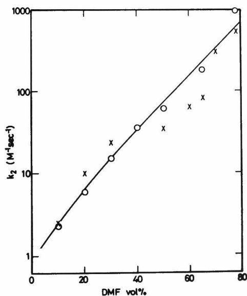
Figure 3 Rate constants of reactions of malachite green with cyanide ion in \text{H}_2\text{O} + DMF mixtures at 25^\circ . [\text{MG}] = 10 \mu\text{M} , [\text{CN}^-] = 10 \text{ mM} , O : UV-SF, × : \kappa -SF
