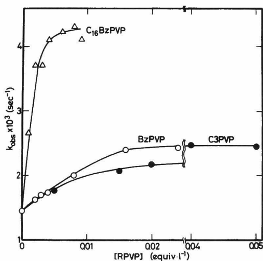
Figure 2 Observed rate constants for the hydrolysis of IAI with varying concentrations of RPVP at 25°C. pH = 10.4, [IAI] = 3.96 \times 10^{-5} \text{M}
