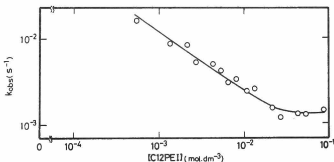
Figure 7 Influence of C12PEI on the alkaline hydrolysis of ANTI in n-hexanol at 25°C. [\text{ANTI}] = 2.50 \times 10^{-5} \text{ M} , [\text{OH}^-] = 1.00 \times 10^{-3} \text{ M} , [\text{H}_2\text{O}] = 5.56 \times 10^{-1} \text{ M}
