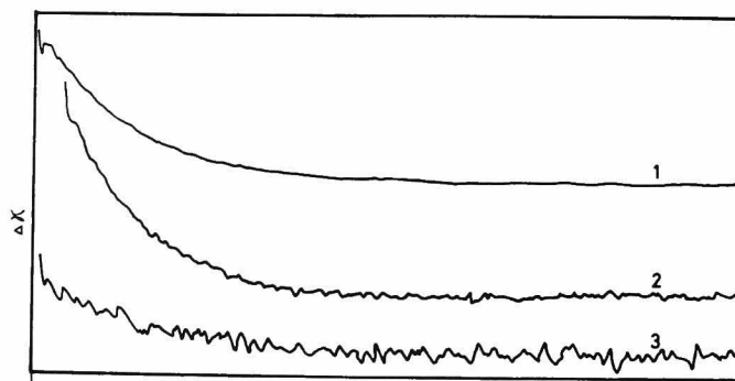
Figure 2 Typical traces of concentration-jump relaxation for \text{Ni}^{2+} -murexide reactions at 25^\circ . [\text{Ni}^{2+}] = 3 \text{ mM} , [\text{murexide}] = 50 \text{ } \mu\text{M} , full scale = 500 msec, curve 1: [\text{KNO}_3] = 0 \text{ M} after mixing, curve 2: [\text{KNO}_3] = 0.01 \text{ M} , curve 3: [\text{KNO}_3] = 0.1 \text{ M}
