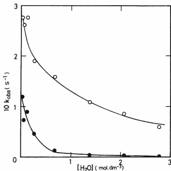
Figure 1. Influence of \text{H}_2\text{O} on the alkaline hydrolysis of PNPA in n-hexanol at 25^\circ\text{C} . [\text{PNPA}] = 2.5 \times 10^{-5}\text{M} , [\text{OH}^-] = 1.00 \times 10^{-3}\text{M} , [\text{C12PEI}] = 0(\text{o}) , 5.51 \times 10^{-3}(\bullet) equiv.l -1
