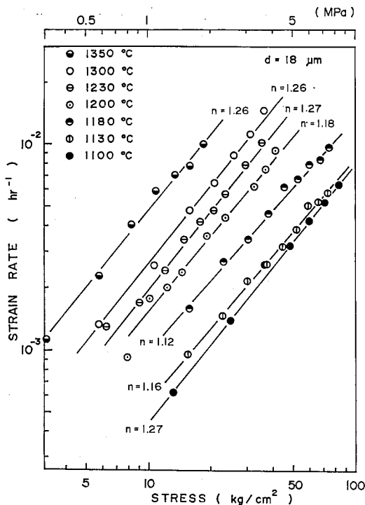
Fig. 1. Stress dependence of strain rate for hot-pressed Mn-Zn ferrite (grain size; d=18 \mu\text{m} ). ( n : stress exponent, \dot{\epsilon} \propto \sigma^n )
