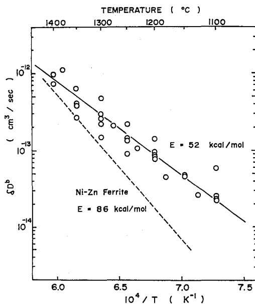
Fig. 4. Apparent grain-boundary diffusivity of oxygen ion in Mn-Zn ferrite, calculated from Eq. (1) for grain sizes between 15 and 80 \mu\text{m} (solid line). Broken line is that for Ni-Zn ferrite with grain sizes between 15 and 30 \mu\text{m} . 4)
