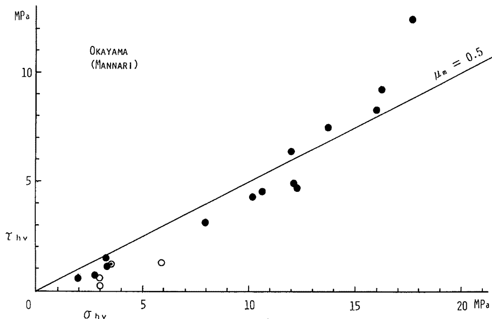
Fig. 6. The ratio ( \mu_m ) of maximum shear stress value to mean stress value considering 3 dimensional stress. Vertical stresses are calculated from theoretical overburden pressure.
