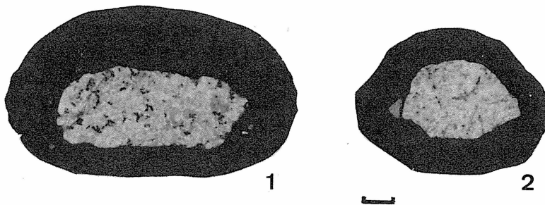
Fig. 1. Granitic rocks obtained at the Komahashi-daini Seamount, Kyushu-Palau Ridge. 1: Biotite granite gravel encrusted with ferro-manganese oxides of ca. 1 cm thick. (GDP-8-12-9) 2: Angular gravel of albite tonalite encrusted with ferro-manganese oxides. (GDP-8-12-12) scale: 1 cm
