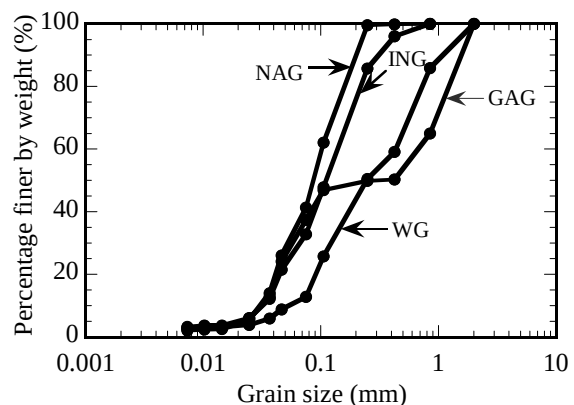
Fig. 1 Grain size distribution curves of the samples
