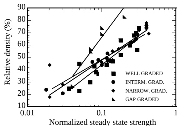
Fig. 3 Normalized steady state strength versus relative density
