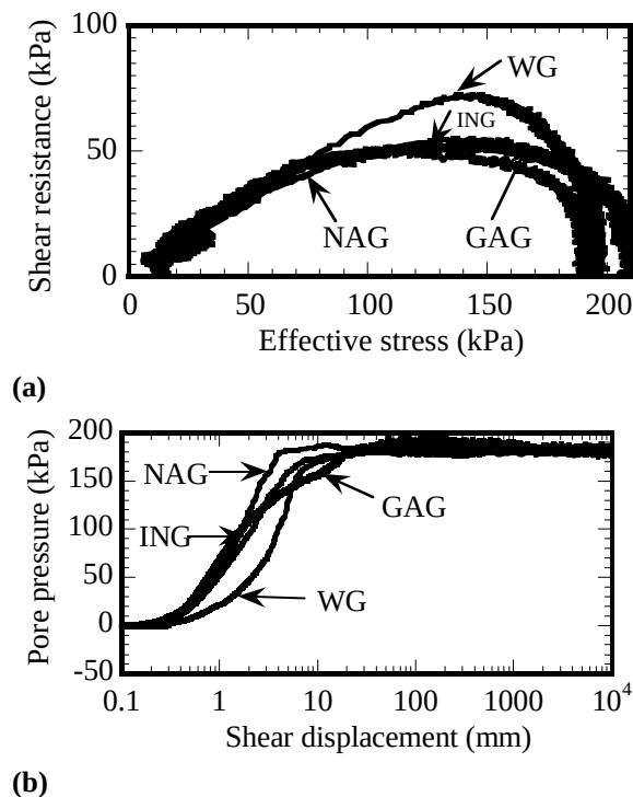
Fig. 6 (a) Stress path (b) Pore pressure evolution
