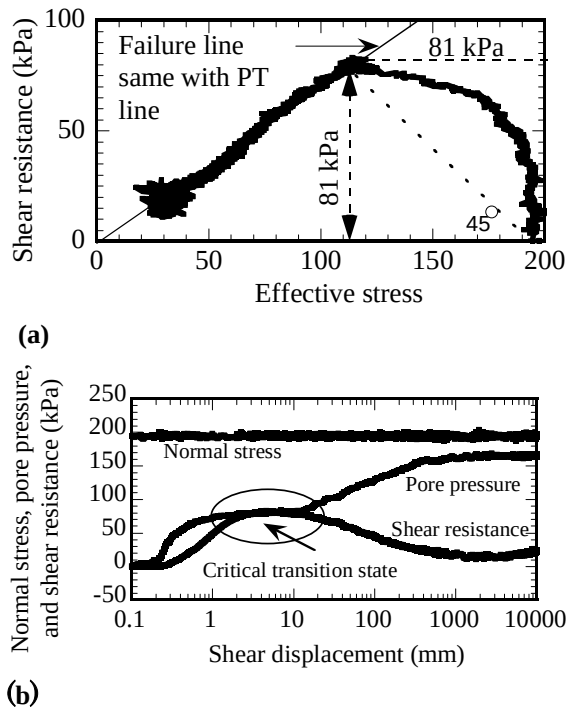
Fig. 9 (a) Stress path defining a critical condition (b) Pore pressure and shear resistance behavior.
