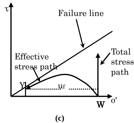
Fig. 8 Schematic diagrams illustrating the concepts of least dilation and critical pore pressure (a) dilation (b) critical (c) liquefaction
