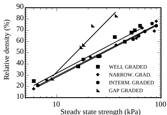
Fig. 5 Steady state strength of specimens confined within a normal stress range of 196 – 202 kPa
