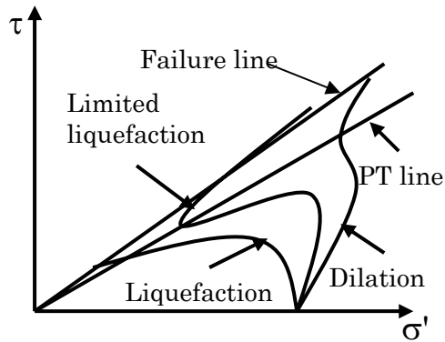
Fig. 7 A sketch of the three basic behaviors of granular materials (after Castro 1969)
