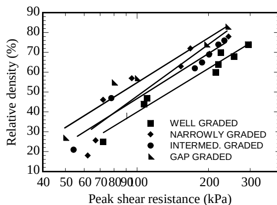
Fig. 4 Peak strength of specimens confined within a normal stress range of 196 – 202 kPa
