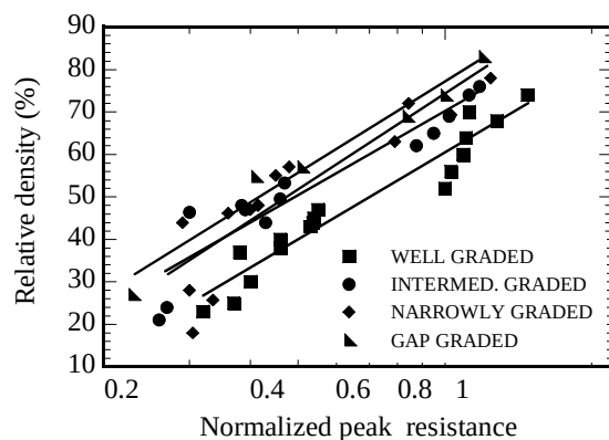
Fig. 2 Normalized peak strength versus relative density
