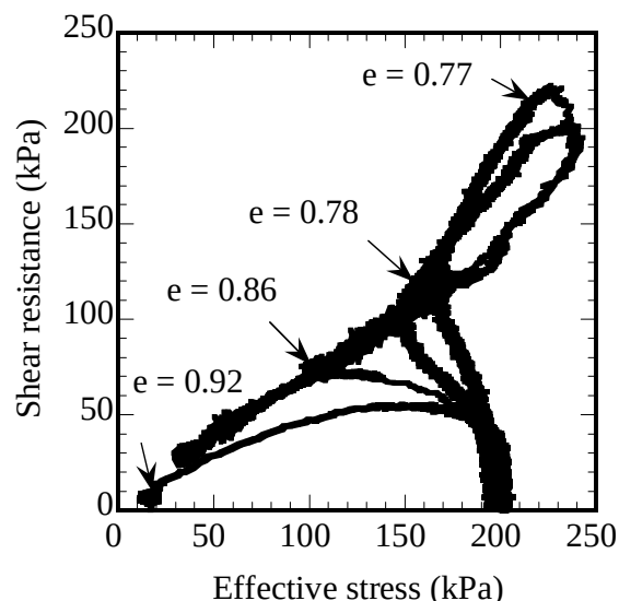
Fig. 14 Stress paths illustrating the influence of density on the behavior of silica sand materials
