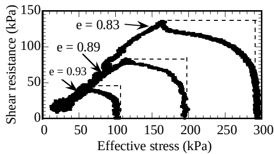
Fig. 12 Critical stress paths of Silica sand specimens
