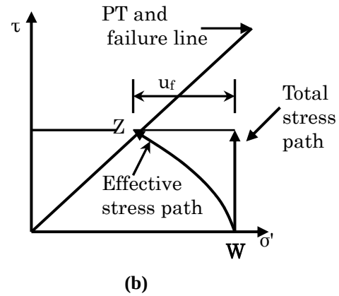
Fig. 7 A sketch of the three basic behaviors of granular materials (after Castro 1969)
