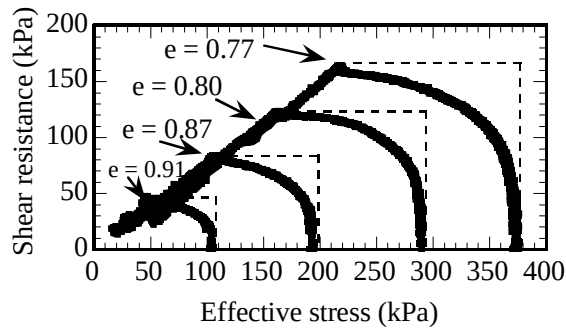
Fig. 11 Critical stress paths of Osaka sand specimens
