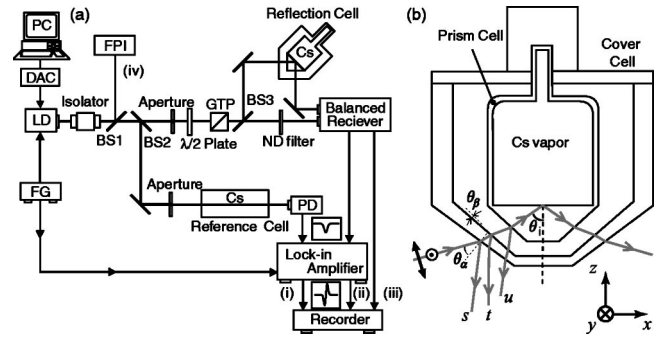
FIG. 6. (a) The experimental setup. LD, laser diode; FPI, Fabry-Pérot interferometer; GTP, Glan-Thompson prism; PD, photodiode; FG, function generator; DAC, digital-analog converter; BS, beam splitter. (b) The geometry of the reflection cell which includes the prism cell and the cover cell.
