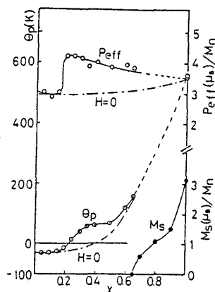
Fig. 2 Ni_{1-x}Mn_xSb の P_{eff}(x), \theta_p(x), M_s(x)
