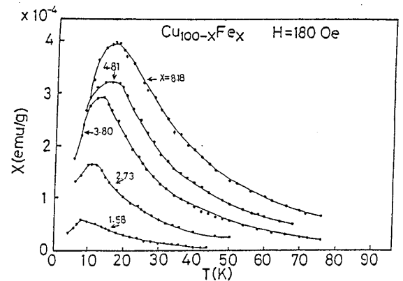
Fig. 10 \text{Cu}_{100-x}\text{Fe}_x の \chi(T)
