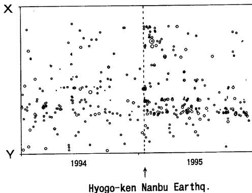
Fig. 4 (c) Time-space distribution of microearthquakes occurred inside the Yamasaki fault area. Dotted line shows the occurrence of the Hyogo-ken nanbu earthquake.
