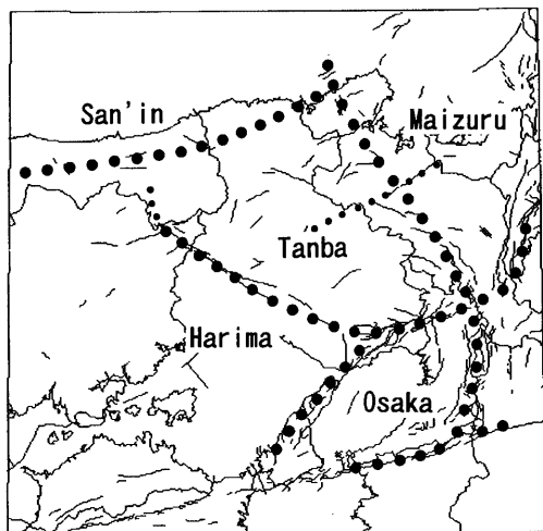
Fig. 2 Block boundaries and active faults. These boundaries were drawn by considering tectonic structure and seismic activity, also being based on those of Katsura et al. 6)
