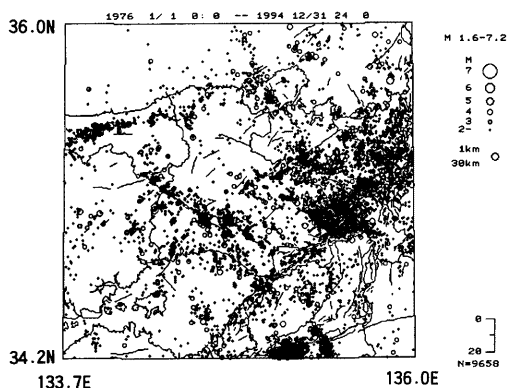
Fig. 1 Epicentral distribution of earthquakes with magnitudes greater than or equal to 1.6 obtained by Tottori network.
