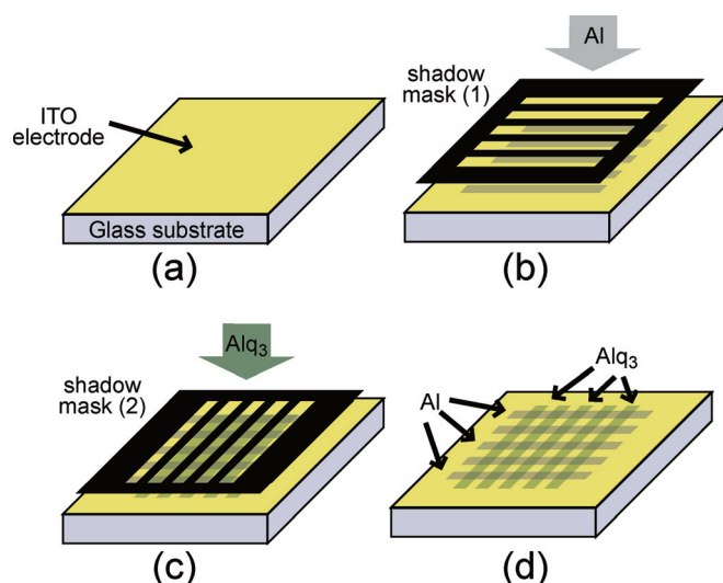
FIG. 1. (Color online) Sample making method. (a) Washing and cleaning (b) Deposition of aluminum using shadow mask (c) Deposition of \text{Alq}_3 using another shadow mask (d) Sample with intersecting area.
