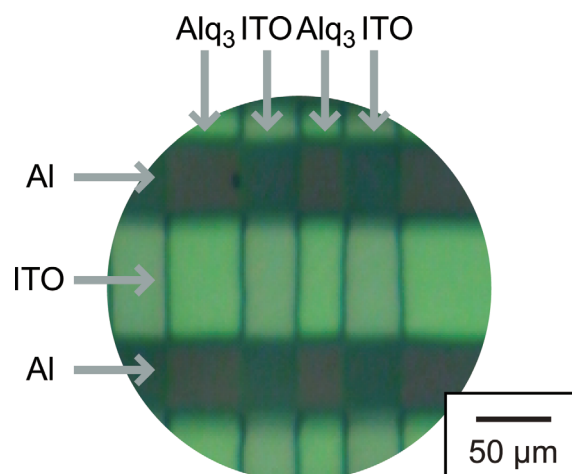
FIG. 2. (Color online) CCD image by optical microscope in DFM of the \text{Alq}_3 and the Al thin films with patterns on the ITO substrate.
