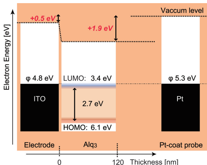
FIG. 5. (Color online) Energy band diagram in the state that the film was formed on ITO electrode.
