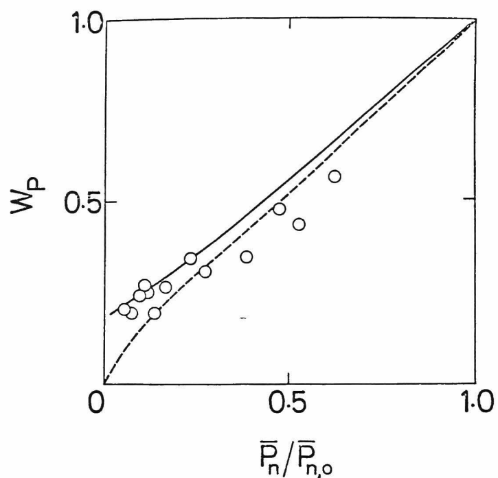
Fig. 9. Plots of weight fraction w_p of PS carrying no transfer agent fragment X against \bar{P}_n/\bar{P}_{n,o} : (o) observed values; (—) calculated according to eq 7; (----) calculated according to eq B7 which is valid for non-degradative transfer.
