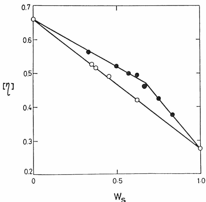
Fig. 1. Dependence of [\eta] on w_s in the polymer mixture for block coupling reaction (polymer conc. = 0.833 g/dl, \bar{M}_n of PS-COCl = 4.51 \times 10^4 and \bar{M}_n of PVAc-NH 2 = 7.56 \times 10^4 ): (o) in the presence of HCl; (•) in the presence of TEA
