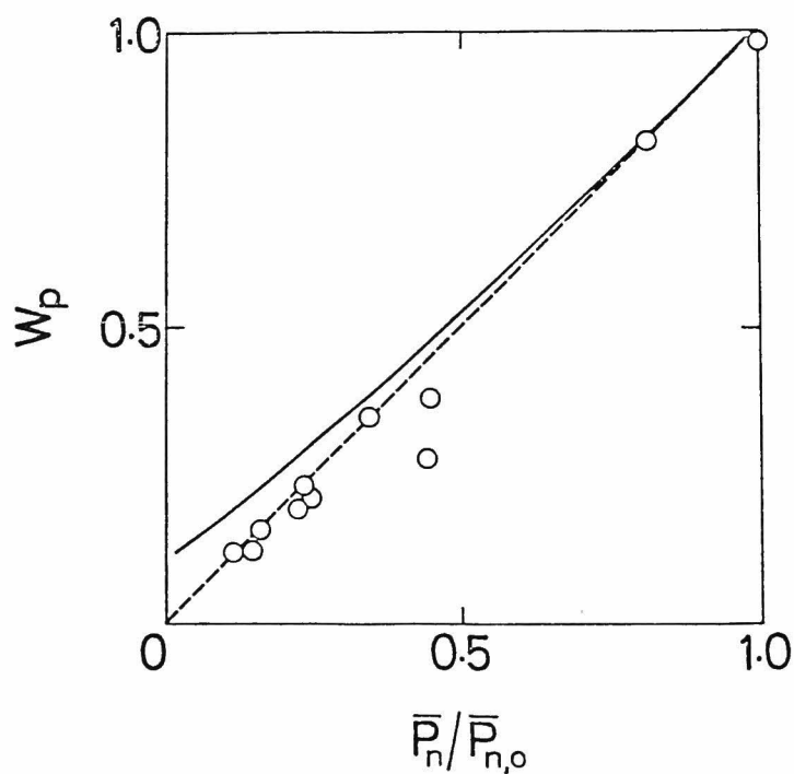
Fig. 10. Plots of weight fraction w_p of PMMA carrying no transfer agent fragment X against \bar{P}_n/\bar{P}_{n,o} : (o) observed values; (—) calculated according to eq 7; (----) calculated according to eq B7 which is valid for non-degradative transfer.
