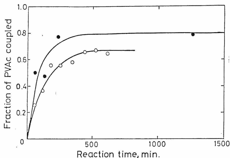
Fig. 4 Reaction of PVAc obtained from \text{IO}_4^- -oxidized PVA with PVA beads (PVAc/PVA=0.5). o [PVAc]=0.461 g·dl -1 , 0.1 N HCl, 60°C; • [PVAc]=0.487 g·dl -1 , 0.4 N H 2 SO 4 , 40°C
