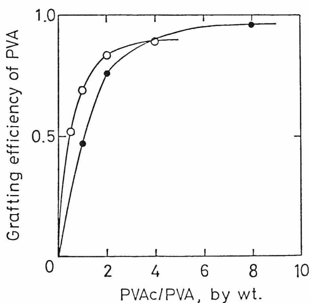
Fig. 9 Dependence of grafting efficiency of PVA on PVAc/PVA ratio (total polymer conc.=5.0 g·dl -1 , 0.1 N HCl, 50°C). o A-5, 19 hr; ● A-6, 28 hr
