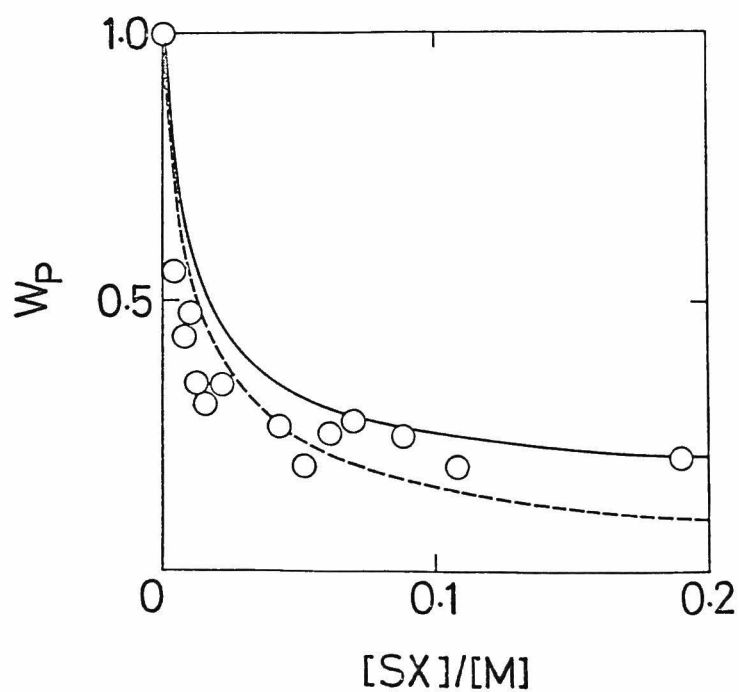
Fig. 7. Plots of weight fraction w_p of PS carrying no transfer agent fragment X against [SX]/[M] : (○) observed values; (—) calculated according to eq 3; (----) calculated according to eq B1 which is valid for non-degradative transfer.
