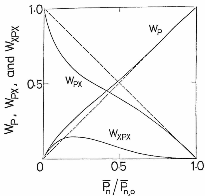
Fig. 12. w_P , w_{PX} , and w_{XPX} values in the case of non-degradative transfer as a function of \bar{P}_n/\bar{P}_{n,o} : (—) \lambda = 0 (coupling termination); (— · —) \lambda = 1 (disproportionation termination).
