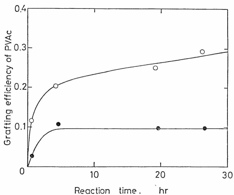
Fig. 7 Dependence of grafting efficiency of PVAc on reaction time for homogeneous reaction ( [PVA]=1.0 \text{ g}\cdot\text{dl}^{-1} ; 0.1 \text{ N HCl} , 50^\circ\text{C} ). o PVAc/PVA=4 (A-5); • PVAc/PVA=8 (B-5)
