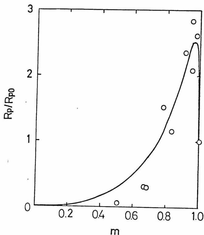
Figure 2 Relative rates of polymerization R_p/R_{p0} of styrene in the presence of trichloroacetyl chloride (TCAC) as a function of the mole fraction of monomer m (dose rate =0.06 \text{ rad}\cdot\text{sec}^{-1} , temp. =50^\circ\text{C} ). \circ observed, — theoretical according to eqs. (A3) and (A11) with \phi_{\text{rel}}=20 and P_{\text{rel}}=30 .
