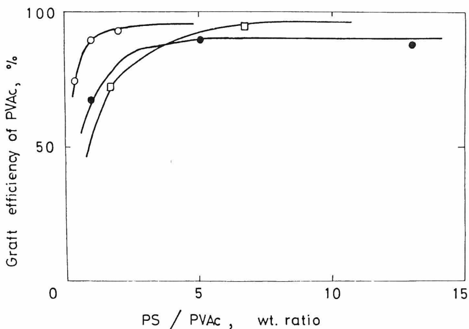
Fig. 6. Influence of polymer weight ratio in feed on graft efficiency of PVAc/NH 2 : (○) \bar{M}_n of PS-COCl = 4.62 \times 10^4 ; (●) \bar{M}_n of PS-COCl = 9.22 \times 10^4 ; (□) \bar{M}_n of PS-COCl = 14.3 \times 10^4 .
