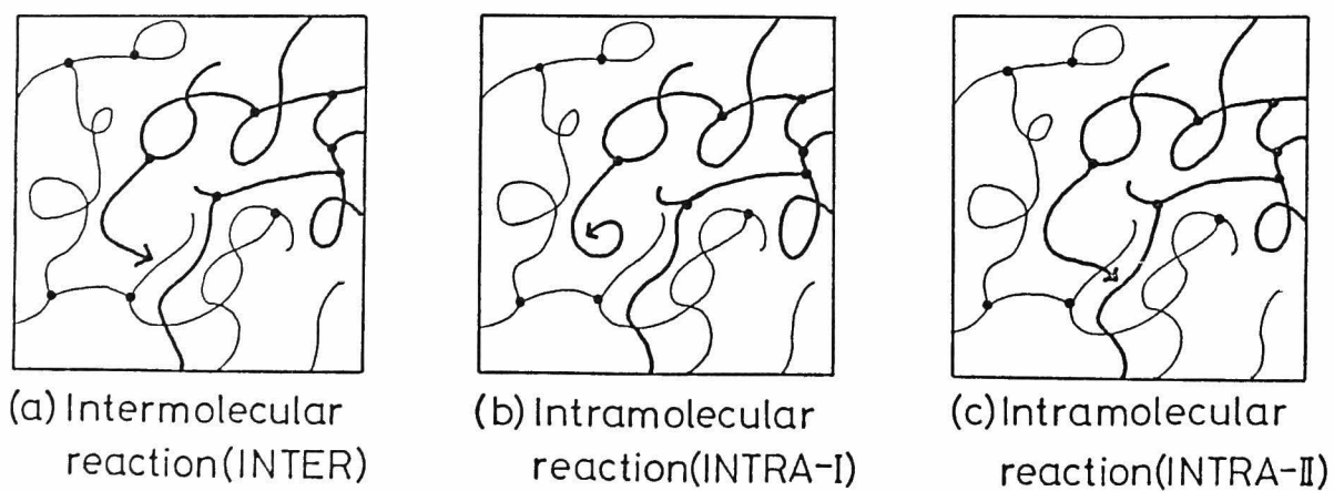
Fig. 5 Schematic representation of inter- and intramolecular reactions.
