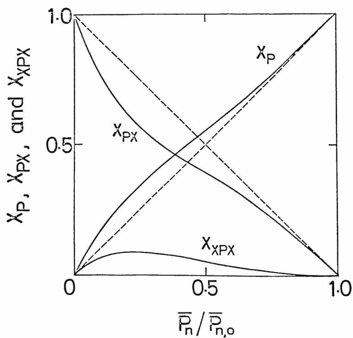
Fig. 13. x_P , x_{PX} , and x_{XPX} values in the case of non-degradative transfer as a function of \bar{P}_n/\bar{P}_{n,o} : (—) \lambda = 0 (coupling termination); (— · —) \lambda = 1 (disproportionation termination).
