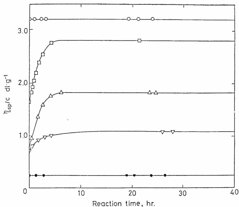
Fig. 2 Variation of solution viscosity with time ( [PVA]=1.0 \text{ g}\cdot\text{dl}^{-1} , 0.1 \text{ N HCl} , 50^\circ\text{C} ). \circ PVA; \bullet PVAc(B-5, [PVAc]=4.0 \text{ g}\cdot\text{dl}^{-1} ); \square PVAc/PVA=4 (A-5); \triangle PVAc/PVA=4 (A-6); \nabla PVAc/PVA=8 (B-5)
