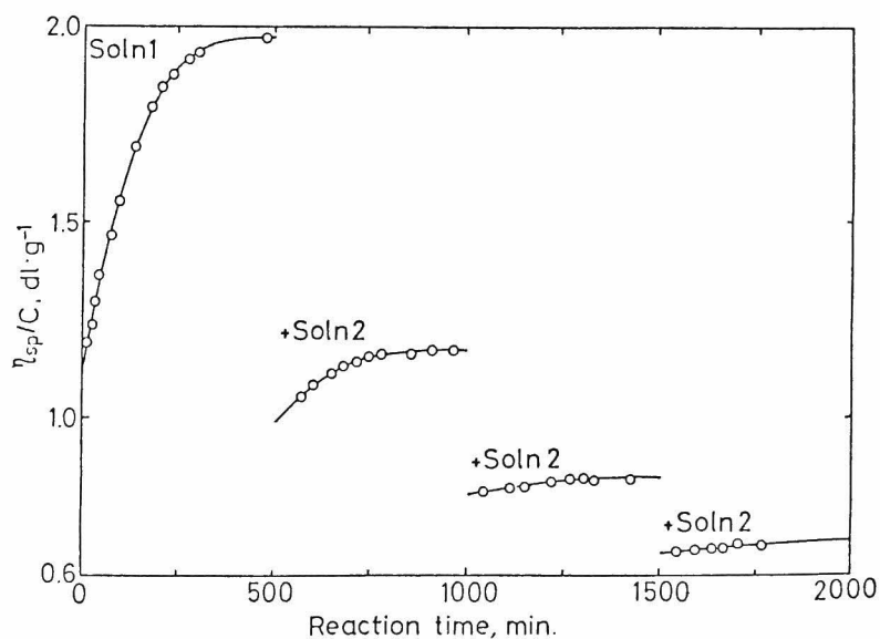
Fig. 3 Variation of solution viscosity accompanying successive addition of PVAc solution(A-2, 0.1 \text{ N HCl} , 50^\circ\text{C} ). Soln 1:PVAc 0.119 \text{ g} , PVA 0.040 \text{ g} , \text{Me}_2\text{SO} 4 \text{ ml} Soln 2:PVAc 0.093 \text{ g} , \text{Me}_2\text{SO} 3 \text{ ml}
