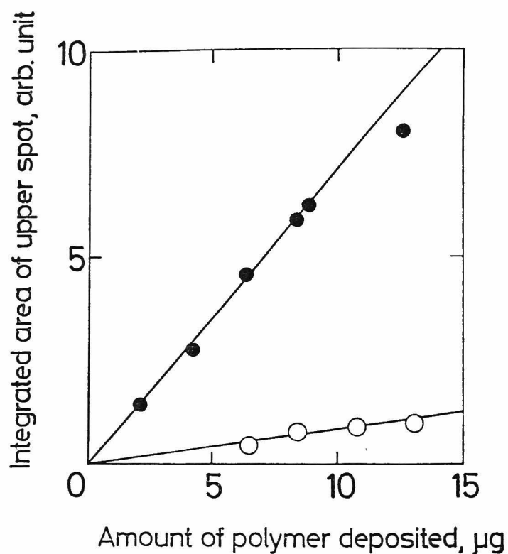
Fig. 6. Relationship between the integrated area of upper spot and the amount of polymer deposited: (○) PMMA, sample number 11; (●) the standard PMMA.
