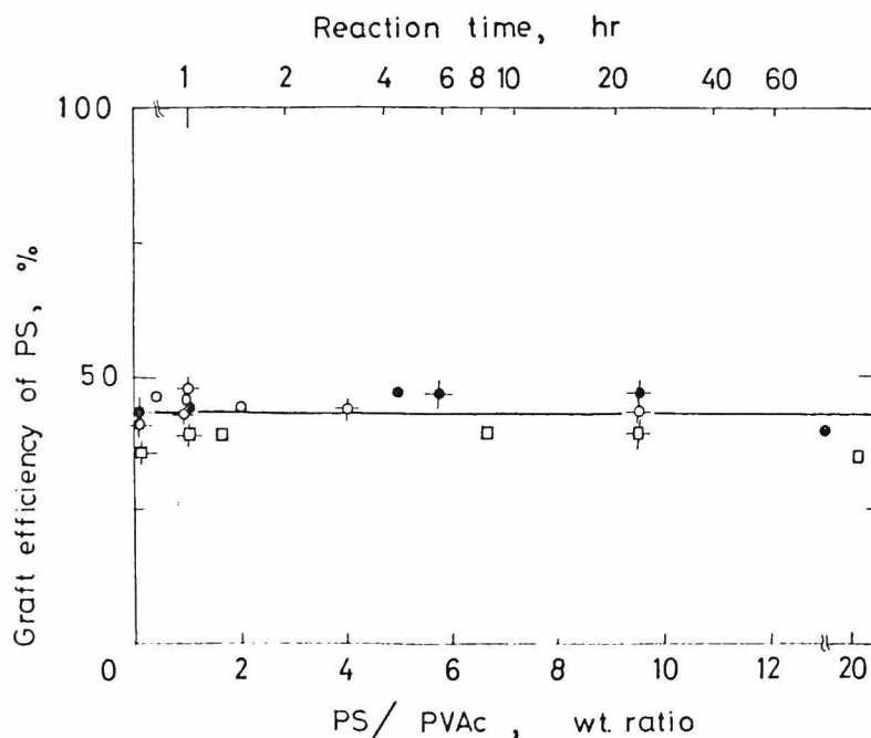
Fig. 5. Influence of polymer weight ratio in feed and reaction time on graft efficiency of PS-COCl: plots for PS/PVAc, (o) \bar{M}_n = 4.62 \times 10^4 , (●) \bar{M}_n = 9.22 \times 10^4 , (□) \bar{M}_n = 14.3 \times 10^4 ; plots for time, (○) \bar{M}_n = 4.62 \times 10^4 , (⊕) \bar{M}_n = 9.22 \times 10^4 , (⊖) \bar{M}_n = 14.3 \times 10^4 .
