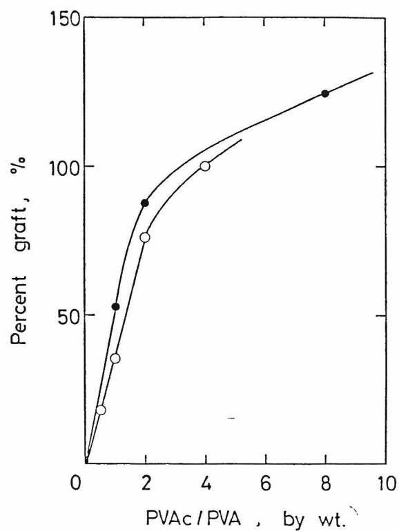
Fig. 8 Dependence of percent graft on PVAc/PVA ratio (total polymer conc.=5.0 g·dl -1 , 0.1 N HCl, 50°C). o A-5, 19 hr, ● A-6, 28 hr
