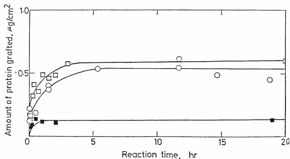
Figure 6 Grafting of various proteins onto DAS-grafted EVA film surfaces (30°C): (□) fibrinogen, 6.7 mg/ml, 0.26 M NaCl, (○) \alpha -amylase, 0.2 mg/ml, 0.01 M \text{Ca}(\text{OAc})_2 , (■) gelatin, 5 mg/ml, 0.05 M NaOH.
