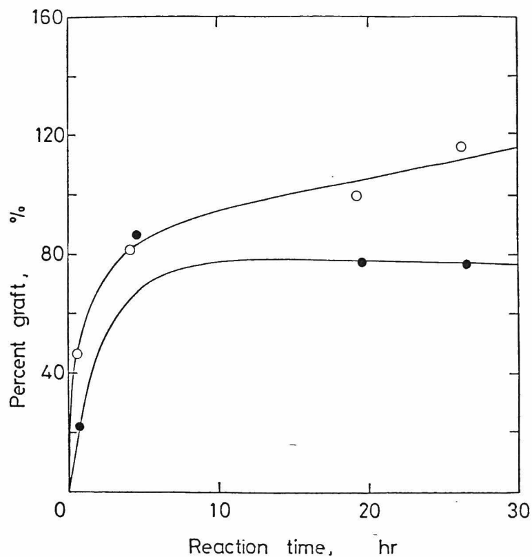
Fig. 6 Dependence of percent graft on reaction time for homogeneous reaction ( [PVA]=1.0 \text{ g}\cdot\text{dl}^{-1} , 0.1 \text{ N HCl} , 50^\circ\text{C} ). o PVAc/PVA=4 (A-5); • PVAc/PVA=8 (B-5)
