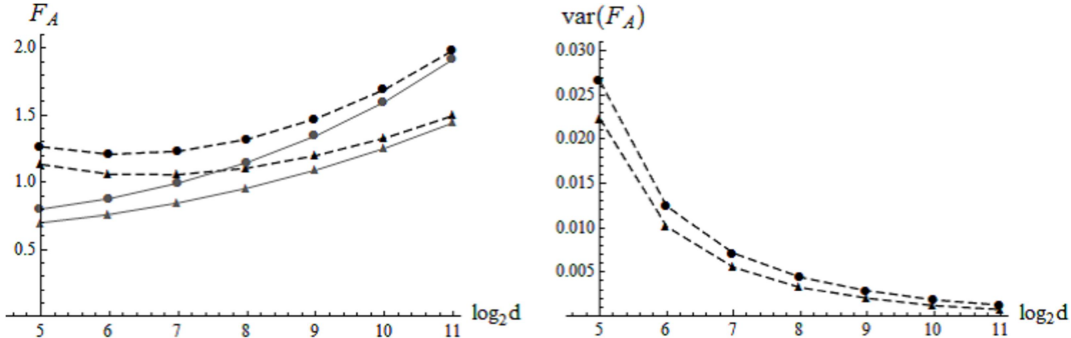
Figure 1: The behaviors of two estimates, \hat{A}_r denoted by \bullet and \check{A}_r denoted by \blacktriangle , when \Sigma_W = I_d . The values of F_{\hat{A}} and F_{\check{A}} are denoted by the dashed lines in the left panel. The values of their sample variances, \text{var}(F_{\hat{A}}) and \text{var}(F_{\check{A}}) , are denoted by the dashed lines in the right panel. The theoretical values, \text{rtr}(\Sigma_W)/(n\lambda_r) and 2 \sum_{i=1}^r \lambda_{i(A)} \{1 - (1 + \kappa_i)^{-1/2}\} / \lambda_r , are denoted by the solid lines in the left panel.
