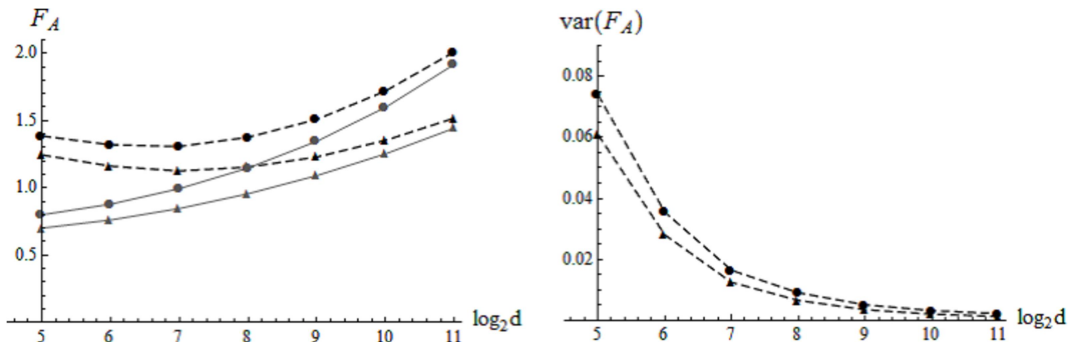
Figure 2: (Continued). When \Sigma_W = (\sigma_{ij}) with \sigma_{ij} = (0.3)^{|i-j|^{1/3}} .
