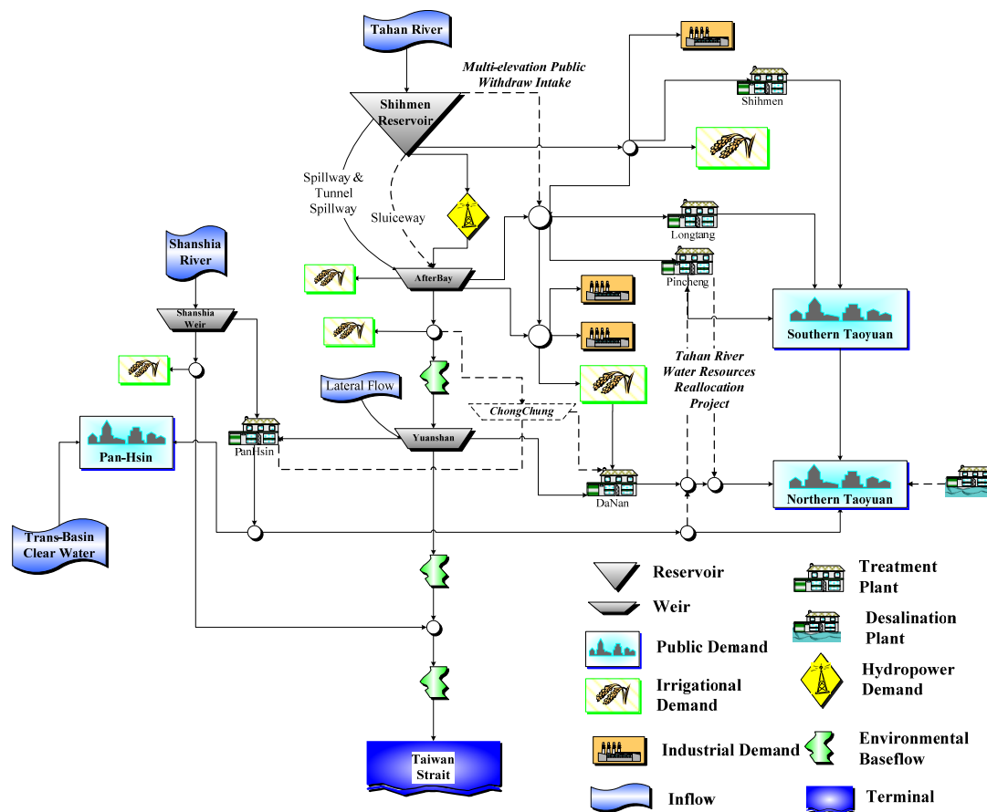
Fig. 2: Network structure of the Tahan River water resources system
