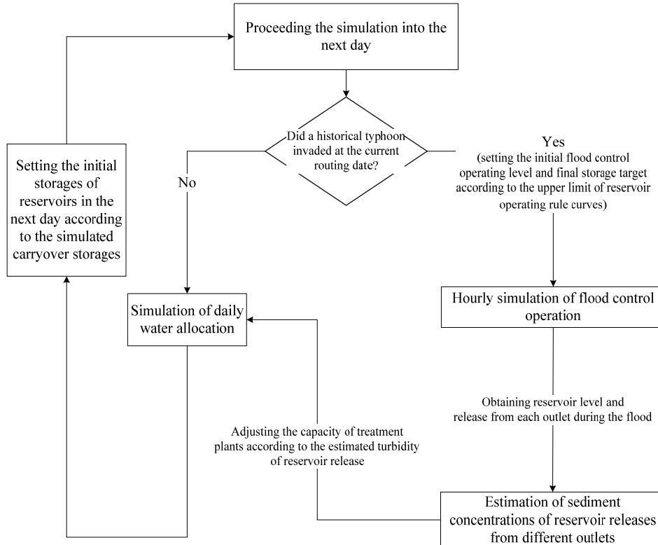
Fig. 1: Integrated framework for joint simulations of regional water supply, reservoir flood control operation and hydraulic sediment routing
