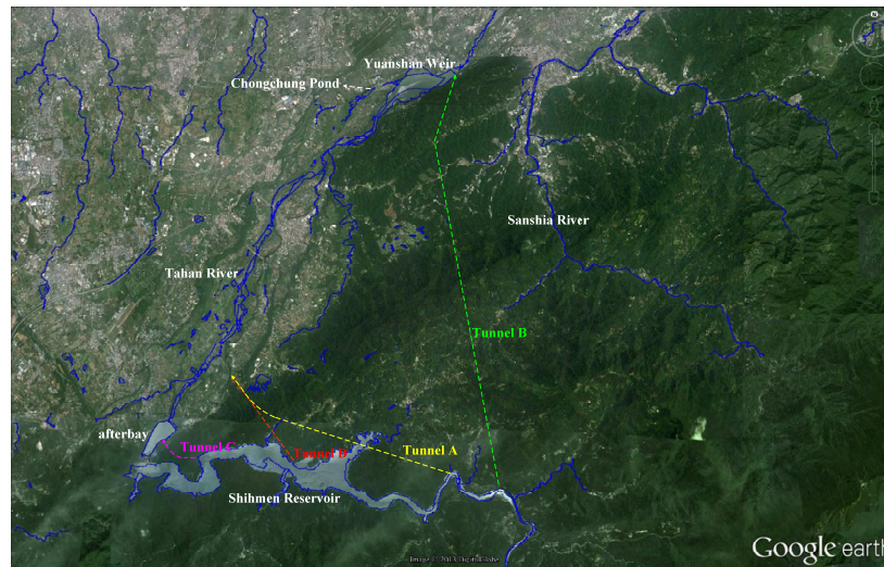
Fig. 4: Locations of sediment routing tunnels
