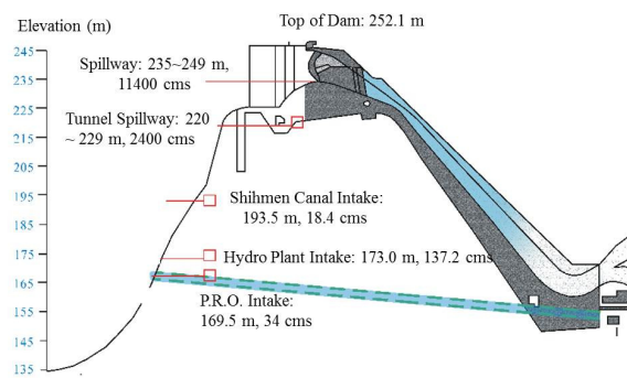
Fig. 3: Major outlets of the Shihmen Reservoir
