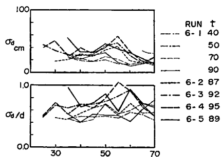
Fig. 6 Deviation of the distance d between watercourses. \bar{d} ; average of the distance d .
