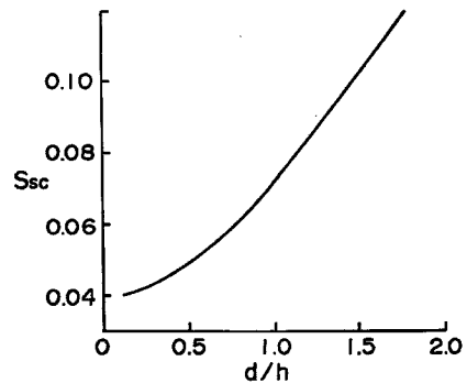
Fig. 15 A diagram for calculation of critical tractive force on particles within shallow flow over inclined slope.
