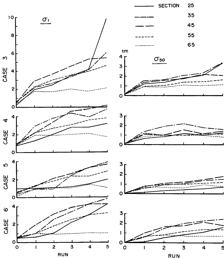
Fig. 11 Variation in deviation of relief.
