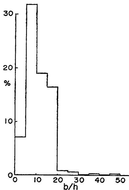
Fig. 8 Histogram of b/h .
