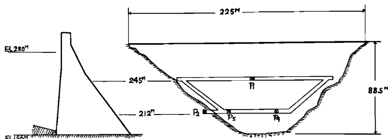
Fig. 31b. Sectional representation of Miyagawa Dam.
