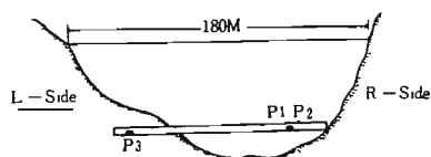
Fig. 40b. Sectional representation of Nagase Dam.
