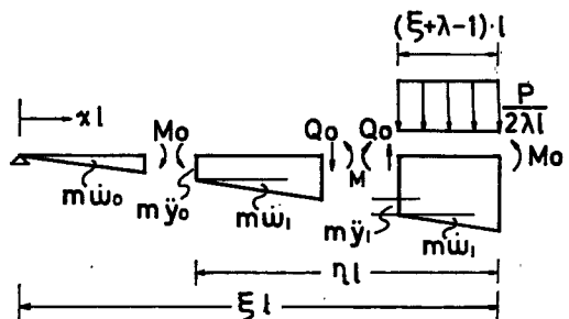
Fig. 12 Type E' Motion
