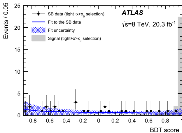
Fig. 5 The distribution of the BDT score of the data in the sideband region (SB) for the tight + x > x_0 selection. The line shows the result of a fit to the BDT score distribution, while the hatched area shows the uncertainty in the fit due to the SB range definition, the x_0 cut location and the fit function choice. The solid grey area shows the signal shape (obtained from MC simulation), normalised to the area of the data for the tight + x > x_0 selection. For illustration, the signal is not constrained to the SR
