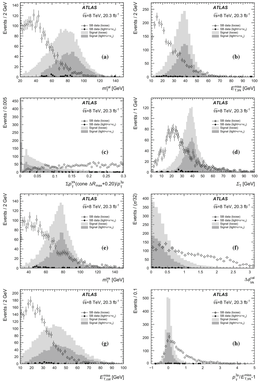
Fig. 2 The BDT inputs ranked 1–8. m_T^{\text{cal}} in a , E_{T,\text{lrk}}^{\text{miss}} in b , \Sigma p_T^{\text{trk}}(\Delta R_{\text{max}}^{3\mu} + 0.20)/p_T^{3\mu} in c , \Sigma_T in d , m_T^{\text{trk}} in e , \Delta\phi_{\text{trk}}^{\text{cal}} in f , E_{T,\text{cal}}^{\text{miss}} in g and p_T^{3\mu}/E_{T,\text{lrk}}^{\text{miss}} - 1 in h . The loose data in the sidebands are shown as hollow circles , while the loose signal MC events are shown as light solid grey area . The tight + x > x_0 data in the sidebands are shown as the solid black circles , while the tight + x > x_0 signal MC events are shown as the
