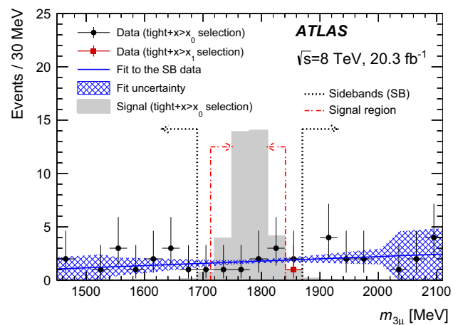
Fig. 6 The three-muon mass distribution in the range [1450, 2110] MeV shown for the tight + x > x_0 selection by solid black circles and for the tight + x > x_1 selection by the solid red square . The sideband and signal regions are indicated by the arrows . The tight + x > x_0 data are fit in the two sidebands simultaneously, excluding the events in the blinded region. The hatched area shows the uncertainty in the fit due to the SB range definition, the x_0 cut location and the fit function choice. The solid grey area shows the signal shape (obtained from MC simulation), normalised to the area of the data for the tight + x > x_0 selection
