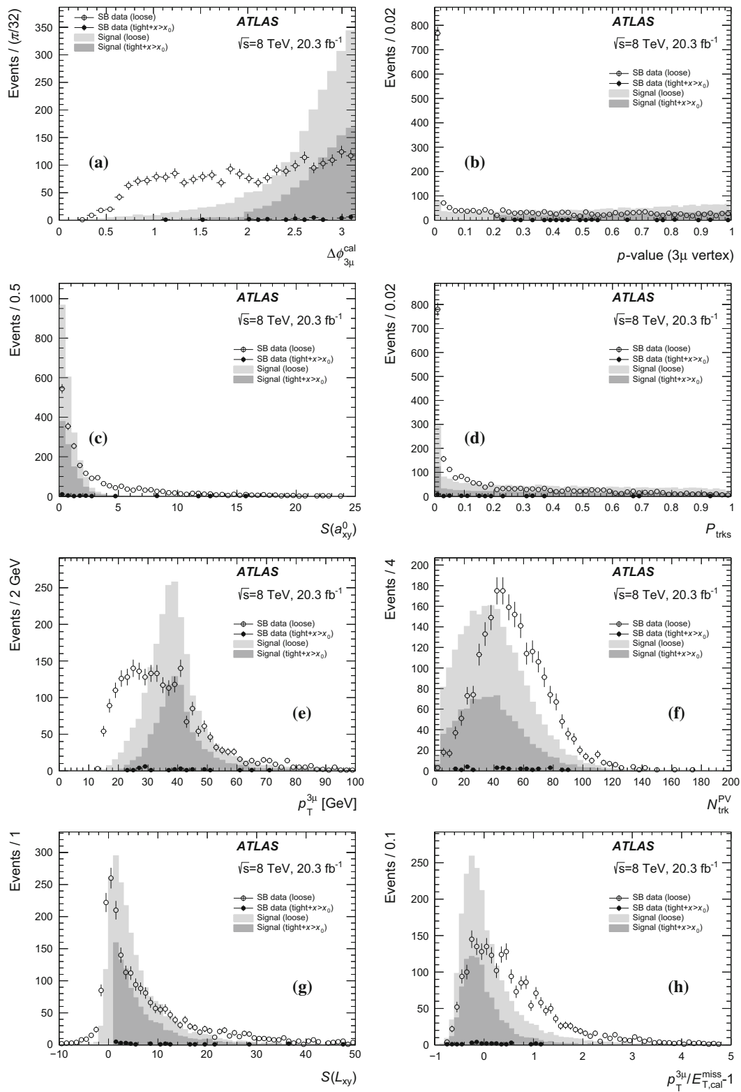
Fig. 3 The BDT inputs ranked 9–16. \Delta\phi_{3\mu}^{\text{cal}} in a , p\text{-value} in b , S(a_{xy}^0) in c , P_{\text{trks}} in d , p_T^{3\mu} in e , N_{\text{trk}}^{\text{PV}} in f , S(L_{xy}) in g and p_T^{3\mu} / E_T^{\text{miss}} - 1 in h . The loose data in the sidebands are shown as hollow circles, while the loose signal MC events are shown as light solid grey area. The tight+x>x _0 data in the sidebands are shown as the solid black circles, while the tight+x>x _0 signal MC events are shown as the dark solid
