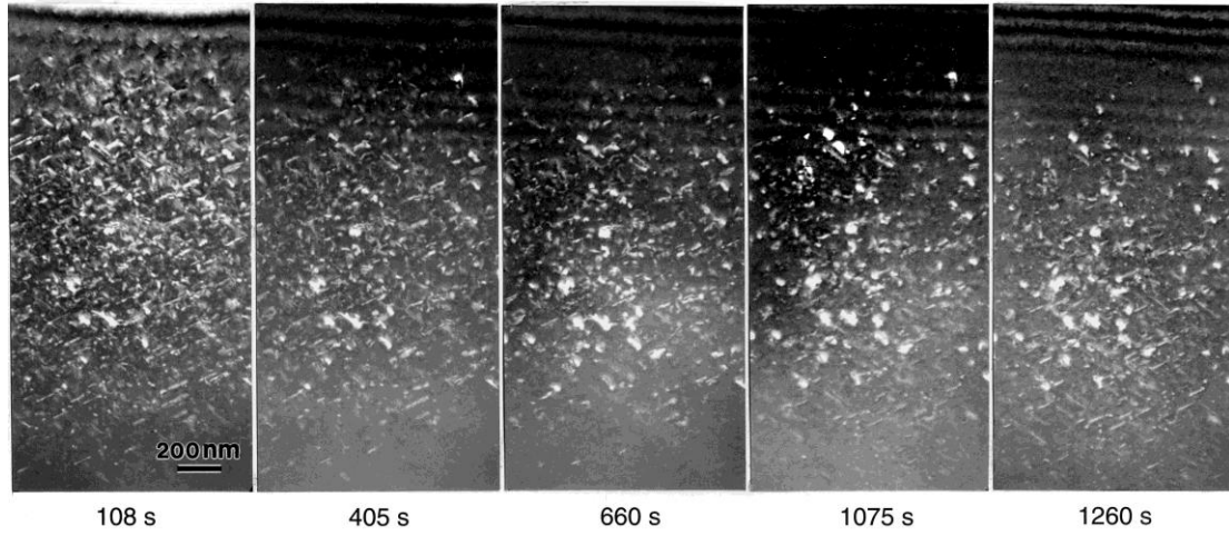
Fig. 5 Growth and shrinkage of {113} interstitial clusters in Fz-Si in two-step irradiation at 623 K under HVEM irradiation. First-step irradiation was for 1800 s. Second-step irradiation from the back side was conducted for the time indicated below each figure at 6 \times 10^{23} \text{ e/m}^2 \cdot \text{s} .
