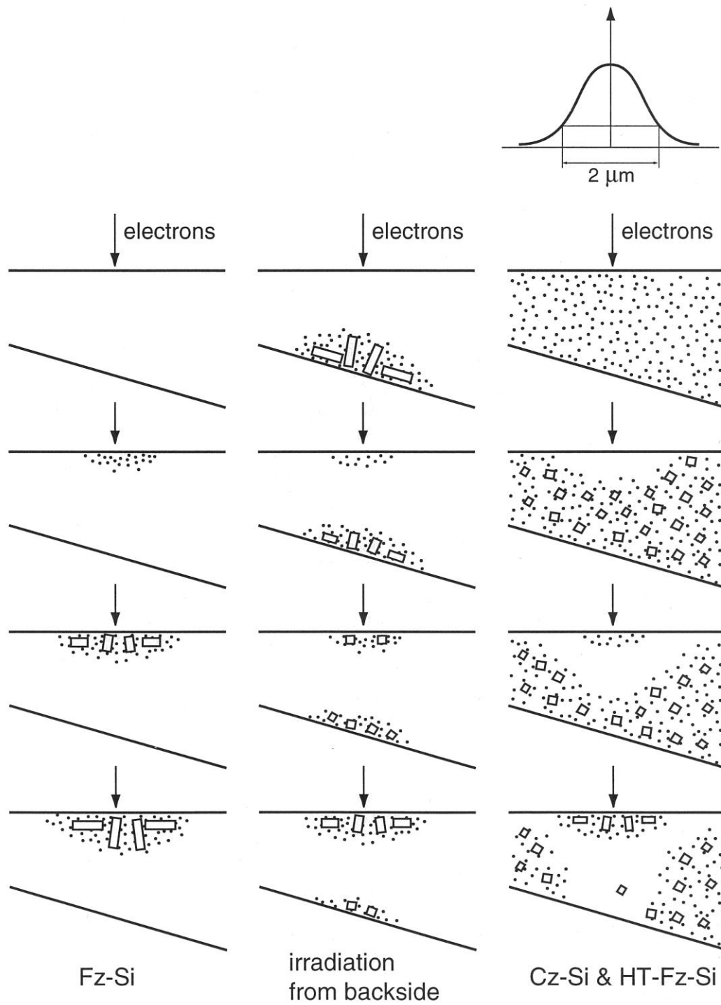
Fig. 10 Schematic illustration of growth and shrinkage behavior of {113} interstitial clusters in Fz-Si (left), backside irradiation of Fz-Si (middle), and HT-Fz-Si and Cz-Si (right). The black dots and rectangles represent impurities and interstitial clusters, respectively.
